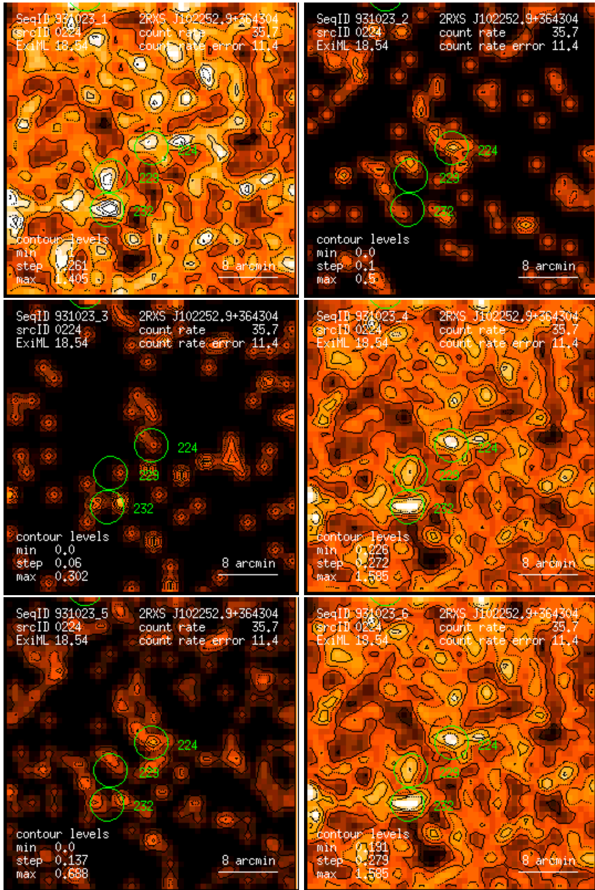
Figure 224: RASS 931023: detection 0224: band rate images, Gaussian filter: (1) PSPC channels 11 – 41, (2) 52 – 90, (3) 91 – 201, (4) 11 – 235, (5) 52 – 201, (6) 11 – 201. Broad band rates in counts/ks. Band rate contour levels in counts/ks/arcmin 2 .
