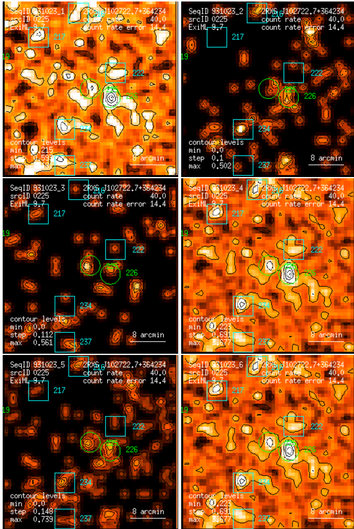
Figure 225: RASS 931023: detection 0225: band rate images, Gaussian filter: (1) PSPC channels 11 – 41, (2) 52 – 90, (3) 91 – 201, (4) 11 – 235, (5) 52 – 201, (6) 11 – 201. Broad band rates in counts/ks. Band rate contour levels in counts/ks/arcmin 2 .
