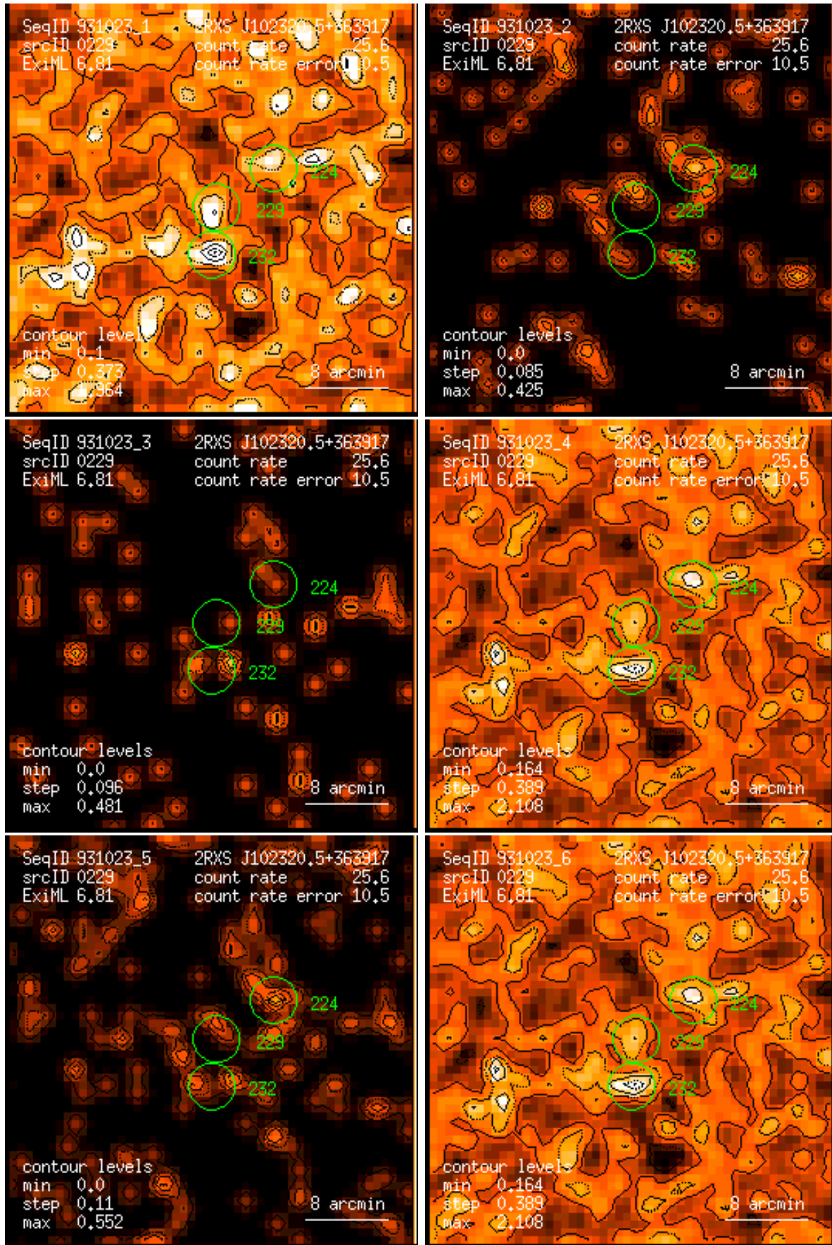
Figure 229: RASS 931023: detection 0229: band rate images, Gaussian filter: (1) PSPC channels 11 – 41, (2) 52 – 90, (3) 91 – 201, (4) 11 – 235, (5) 52 – 201, (6) 11 – 201. Broad band rates in counts/ks. Band rate contour levels in counts/ks/arcmin 2 .
