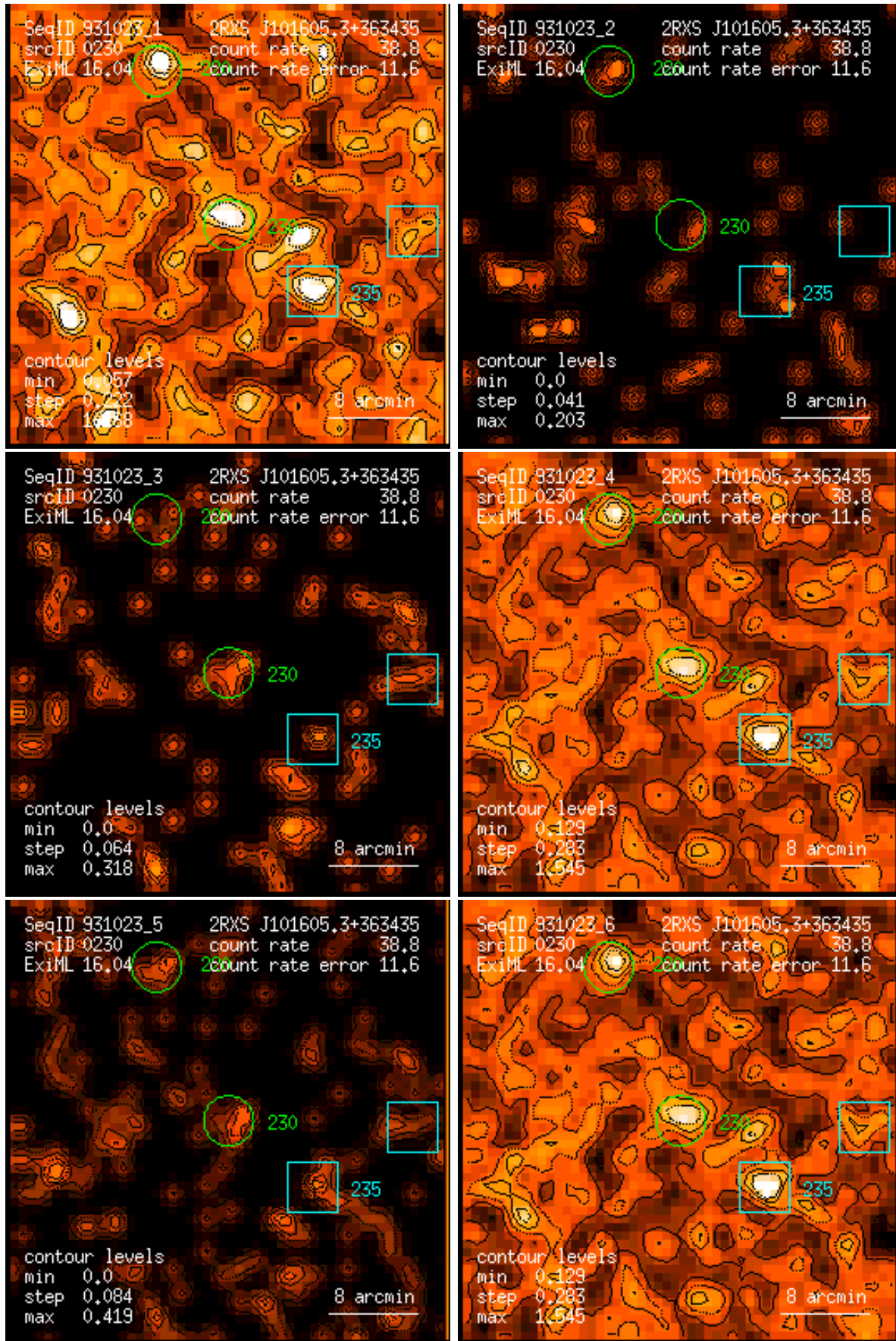
Figure 230: RASS 931023: detection 0230: band rate images, Gaussian filter: (1) PSPC channels 11 – 41, (2) 52 – 90, (3) 91 – 201, (4) 11 – 235, (5) 52 – 201, (6) 11 – 201. Broad band rates in counts/ks. Band rate contour levels in counts/ks/arcmin 2 .
