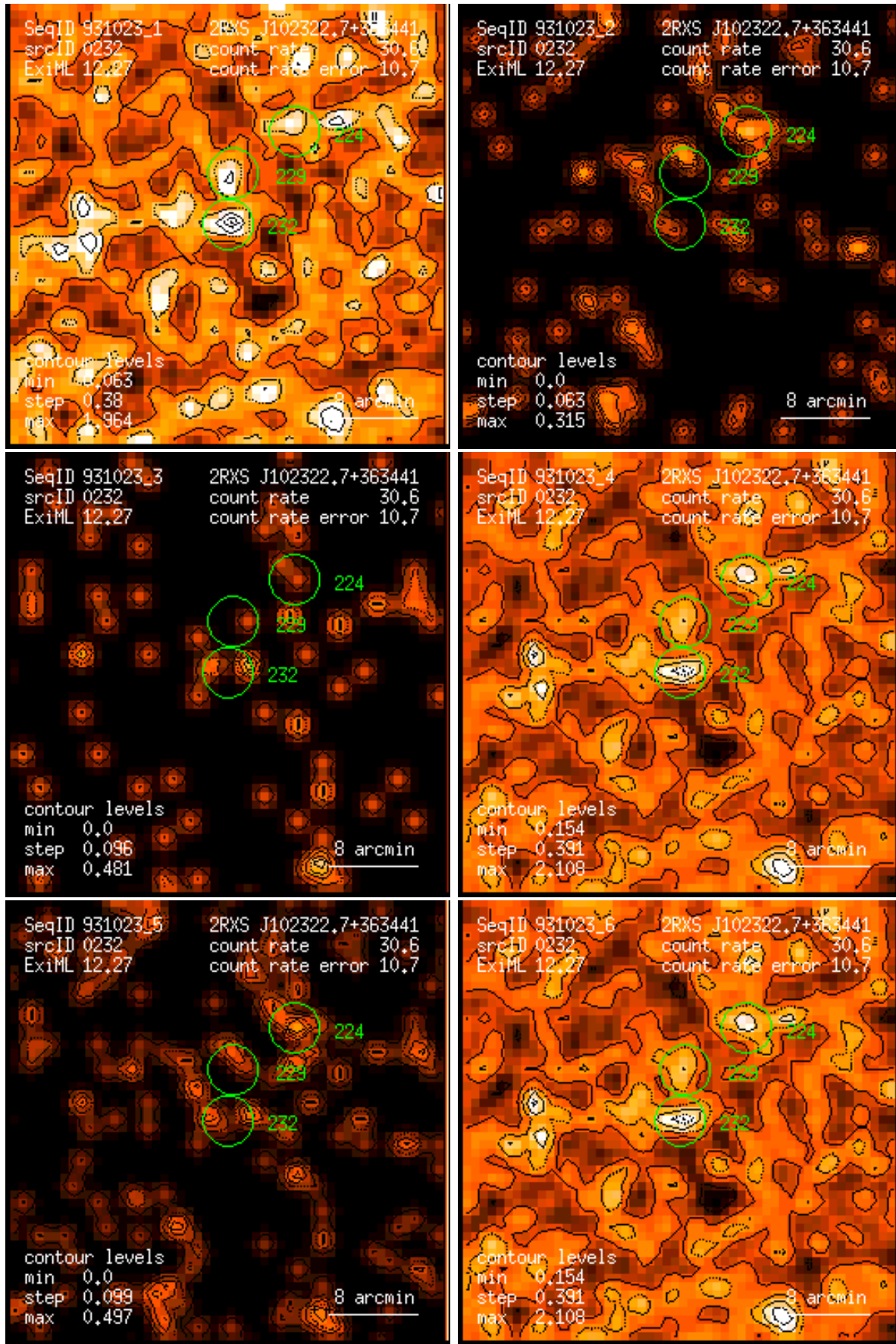
Figure 232: RASS 931023: detection 0232: band rate images, Gaussian filter: (1) PSPC channels 11 – 41, (2) 52 – 90, (3) 91 – 201, (4) 11 – 235, (5) 52 – 201, (6) 11 – 201. Broad band rates in counts/ks. Band rate contour levels in counts/ks/arcmin 2 .
