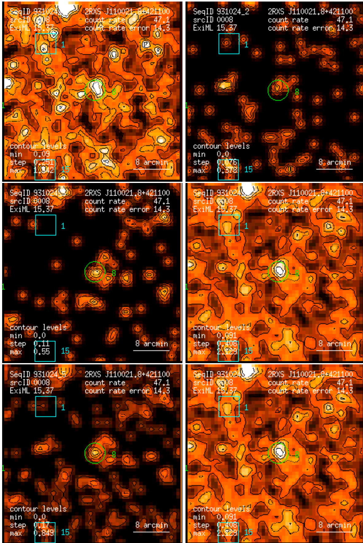
Figure 8: RASS 931024: detection 0008: band rate images, Gaussian filter: (1) PSPC channels 11 – 41, (2) 52 – 90, (3) 91 – 201, (4) 11 – 235, (5) 52 – 201, (6) 11 – 201. Broad band rates in counts/ks. Band rate contour levels in counts/ks/arcmin 2 .
