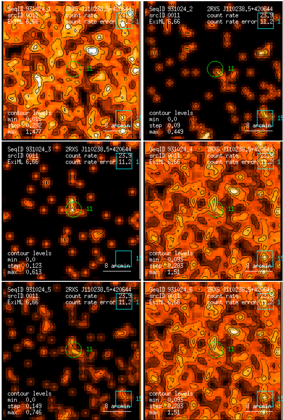
Figure 11: RASS 931024: detection 0011: band rate images, Gaussian filter: (1) PSPC channels 11 – 41, (2) 52 – 90, (3) 91 – 201, (4) 11 – 235, (5) 52 – 201, (6) 11 – 201. Broad band rates in counts/ks. Band rate contour levels in counts/ks/arcmin 2 .
