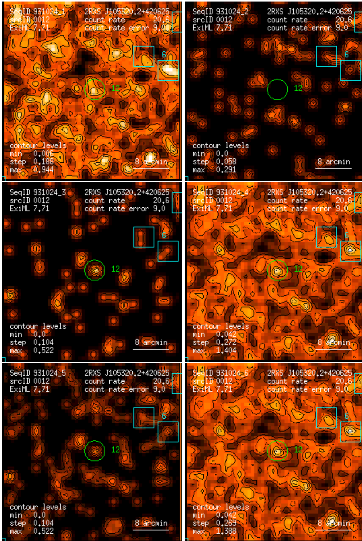
Figure 12: RASS 931024: detection 0012: band rate images, Gaussian filter: (1) PSPC channels 11 – 41, (2) 52 – 90, (3) 91 – 201, (4) 11 – 235, (5) 52 – 201, (6) 11 – 201. Broad band rates in counts/ks. Band rate contour levels in counts/ks/arcmin 2 .
