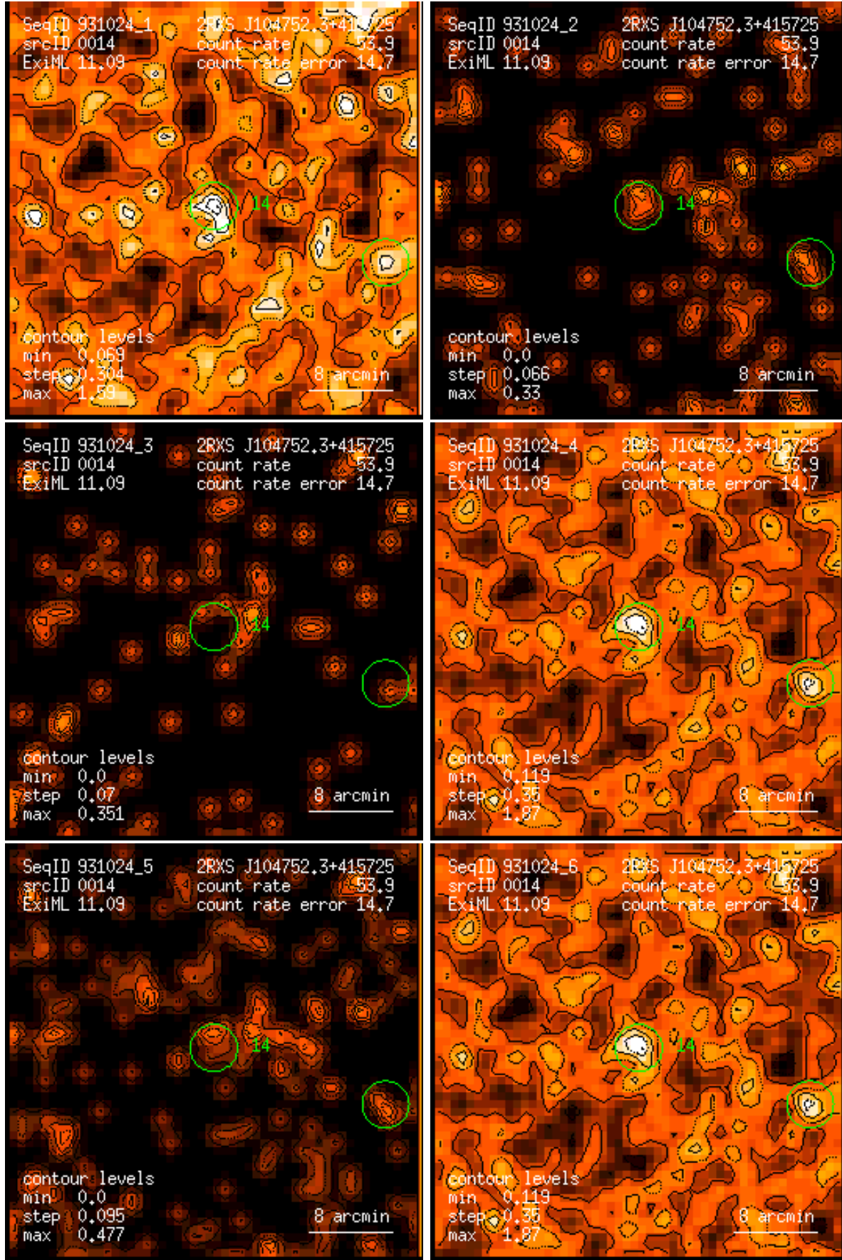
Figure 14: RASS 931024: detection 0014: band rate images, Gaussian filter: (1) PSPC channels 11 – 41, (2) 52 – 90, (3) 91 – 201, (4) 11 – 235, (5) 52 – 201, (6) 11 – 201. Broad band rates in counts/ks. Band rate contour levels in counts/ks/arcmin 2 .
