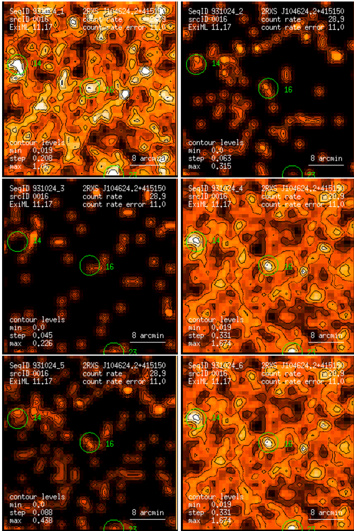
Figure 16: RASS 931024: detection 0016: band rate images, Gaussian filter: (1) PSPC channels 11 – 41, (2) 52 – 90, (3) 91 – 201, (4) 11 – 235, (5) 52 – 201, (6) 11 – 201. Broad band rates in counts/ks. Band rate contour levels in counts/ks/arcmin 2 .
