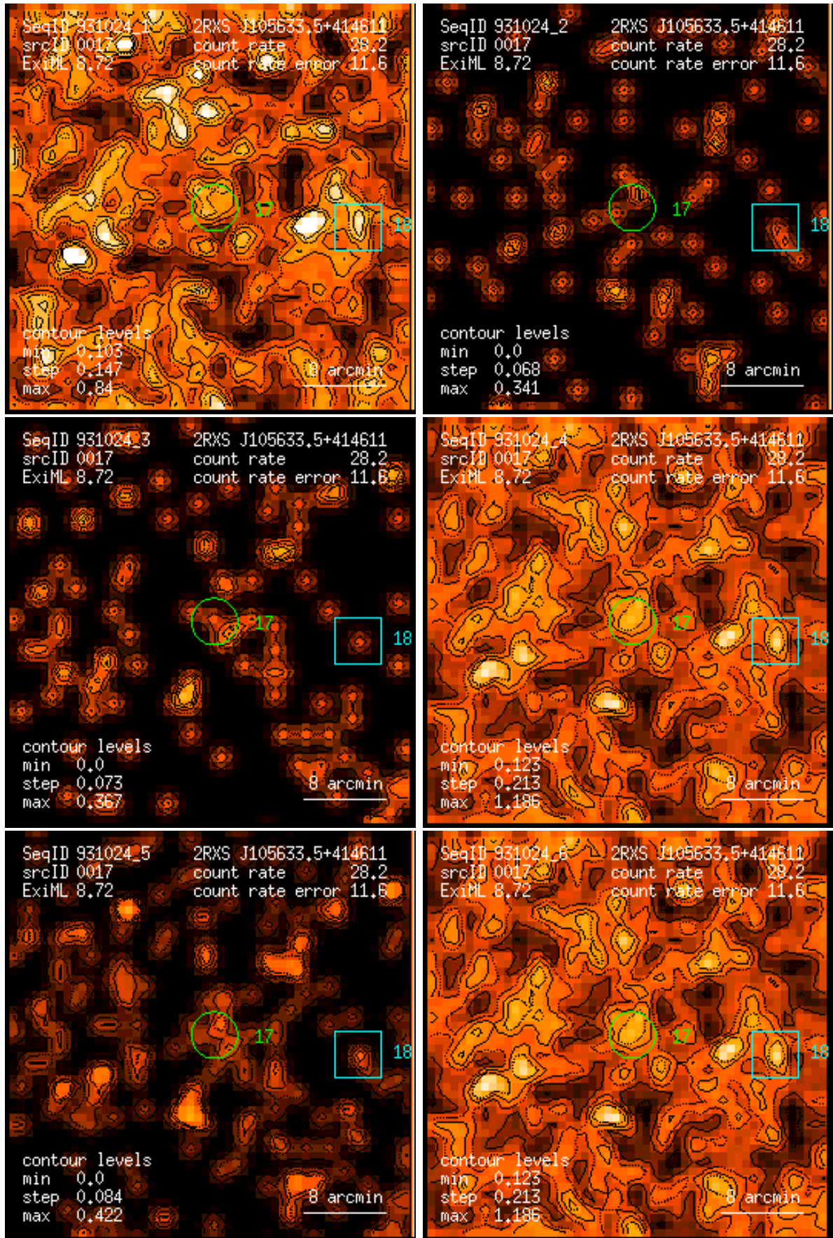
Figure 17: RASS 931024: detection 0017: band rate images, Gaussian filter: (1) PSPC channels 11 – 41, (2) 52 – 90, (3) 91 – 201, (4) 11 – 235, (5) 52 – 201, (6) 11 – 201. Broad band rates in counts/ks. Band rate contour levels in counts/ks/arcmin 2 .
