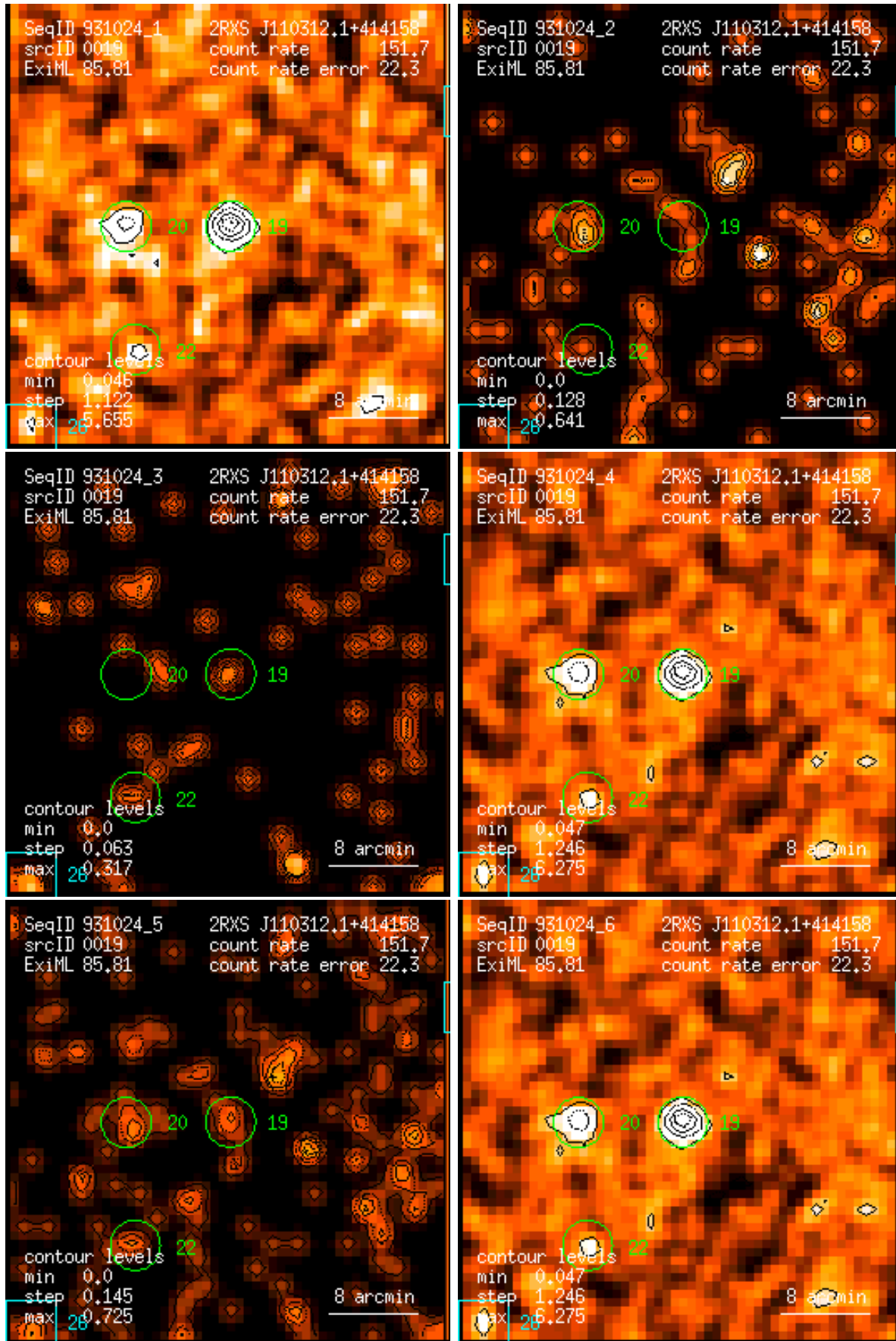
Figure 19: RASS 931024: detection 0019: band rate images, Gaussian filter: (1) PSPC channels 11 – 41, (2) 52 – 90, (3) 91 – 201, (4) 11 – 235, (5) 52 – 201, (6) 11 – 201. Broad band rates in counts/ks. Band rate contour levels in counts/ks/arcmin 2 .
