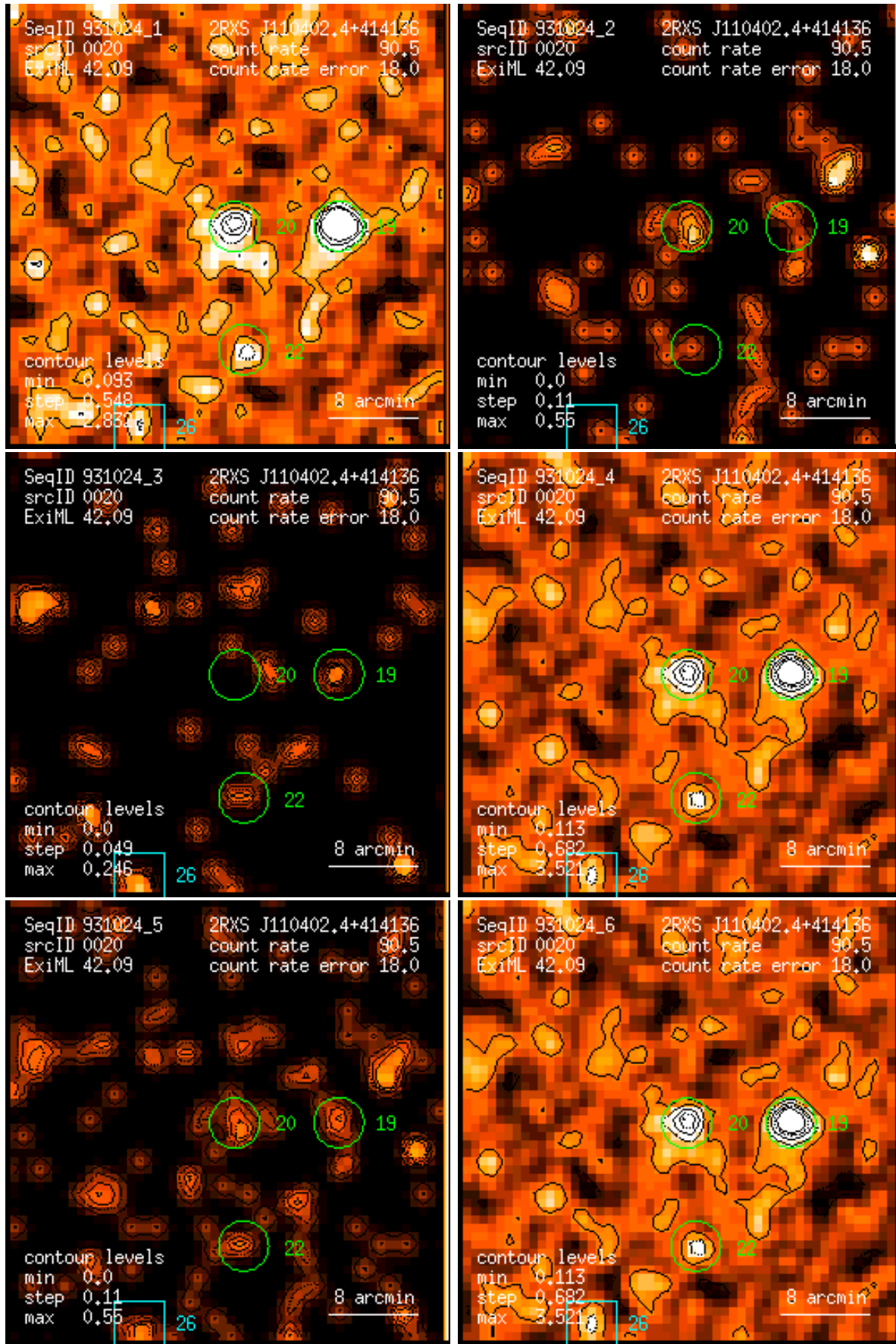
Figure 20: RASS 931024: detection 0020: band rate images, Gaussian filter: (1) PSPC channels 11 – 41, (2) 52 – 90, (3) 91 – 201, (4) 11 – 235, (5) 52 – 201, (6) 11 – 201. Broad band rates in counts/ks. Band rate contour levels in counts/ks/arcmin 2 .
