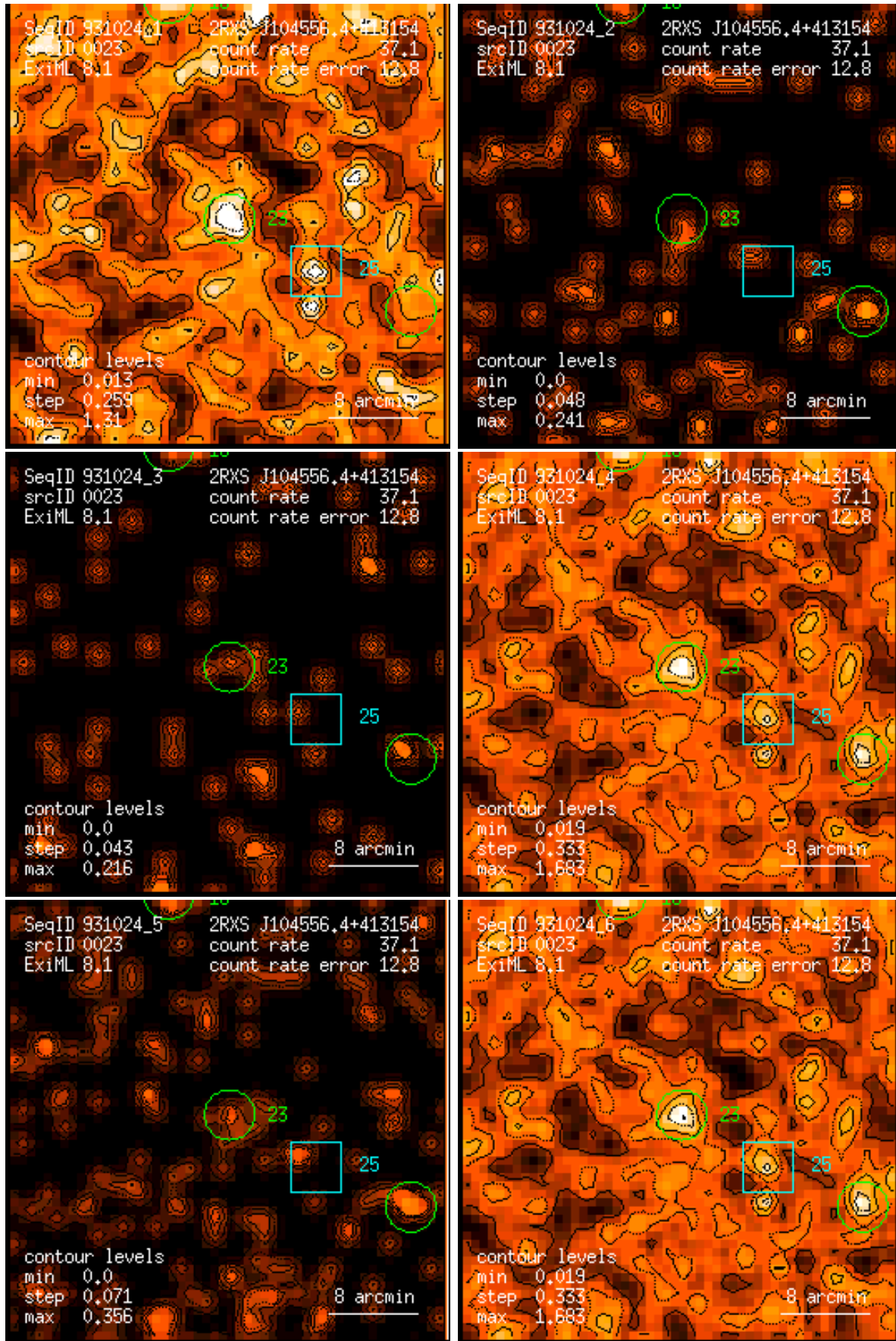
Figure 23: RASS 931024: detection 0023: band rate images, Gaussian filter: (1) PSPC channels 11 – 41, (2) 52 – 90, (3) 91 – 201, (4) 11 – 235, (5) 52 – 201, (6) 11 – 201. Broad band rates in counts/ks. Band rate contour levels in counts/ks/arcmin 2 .
