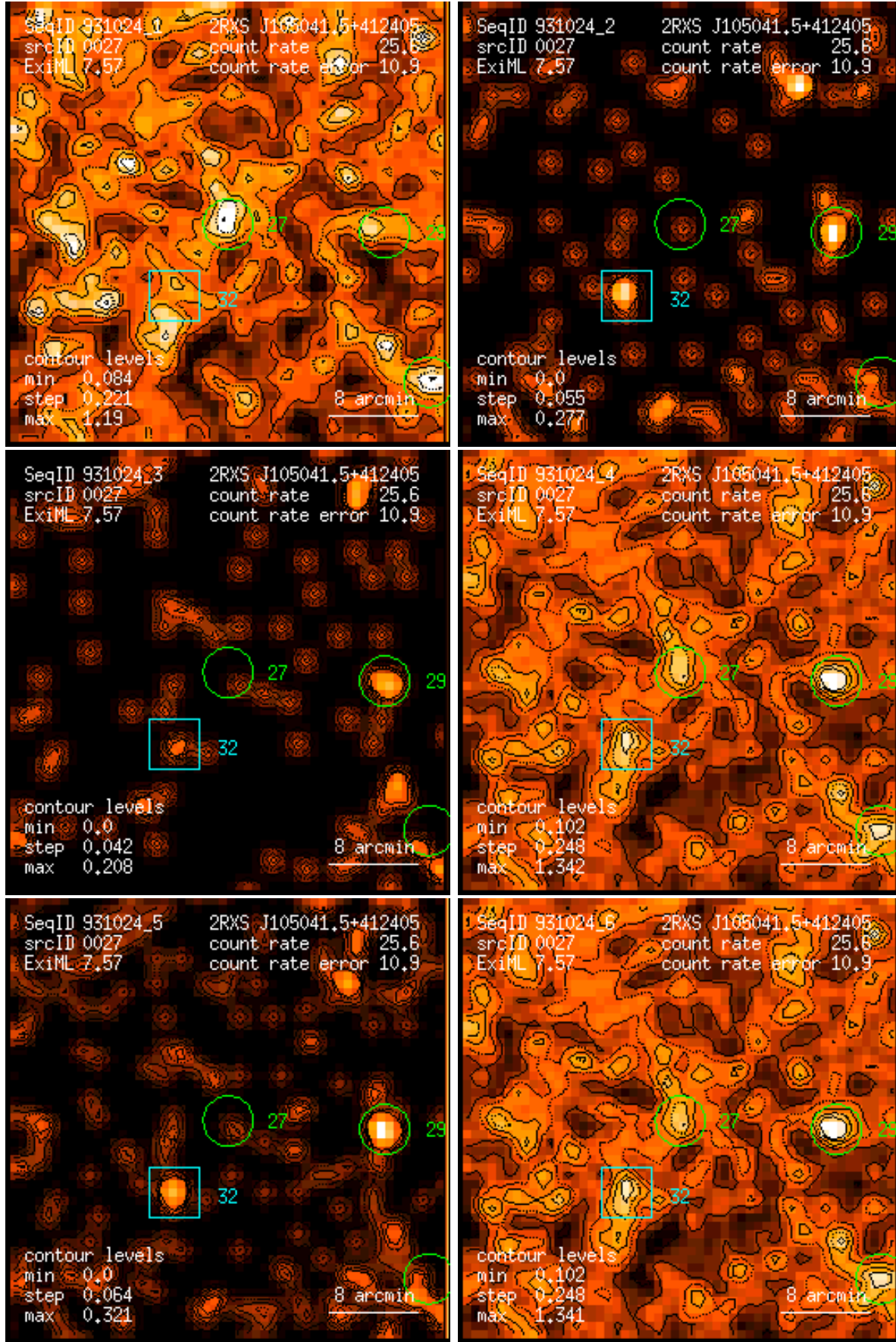
Figure 27: RASS 931024: detection 0027: band rate images, Gaussian filter: (1) PSPC channels 11 – 41, (2) 52 – 90, (3) 91 – 201, (4) 11 – 235, (5) 52 – 201, (6) 11 – 201. Broad band rates in counts/ks. Band rate contour levels in counts/ks/arcmin 2 .
