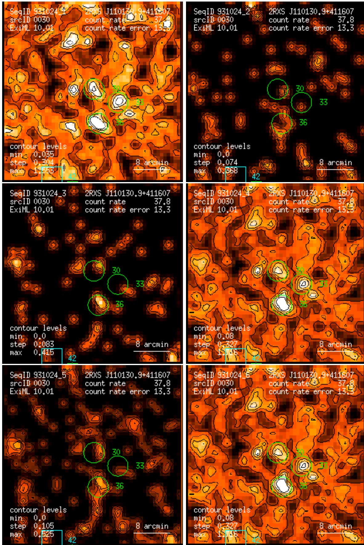
Figure 30: RASS 931024: detection 0030: band rate images, Gaussian filter: (1) PSPC channels 11 – 41, (2) 52 – 90, (3) 91 – 201, (4) 11 – 235, (5) 52 – 201, (6) 11 – 201. Broad band rates in counts/ks. Band rate contour levels in counts/ks/arcmin 2 .
