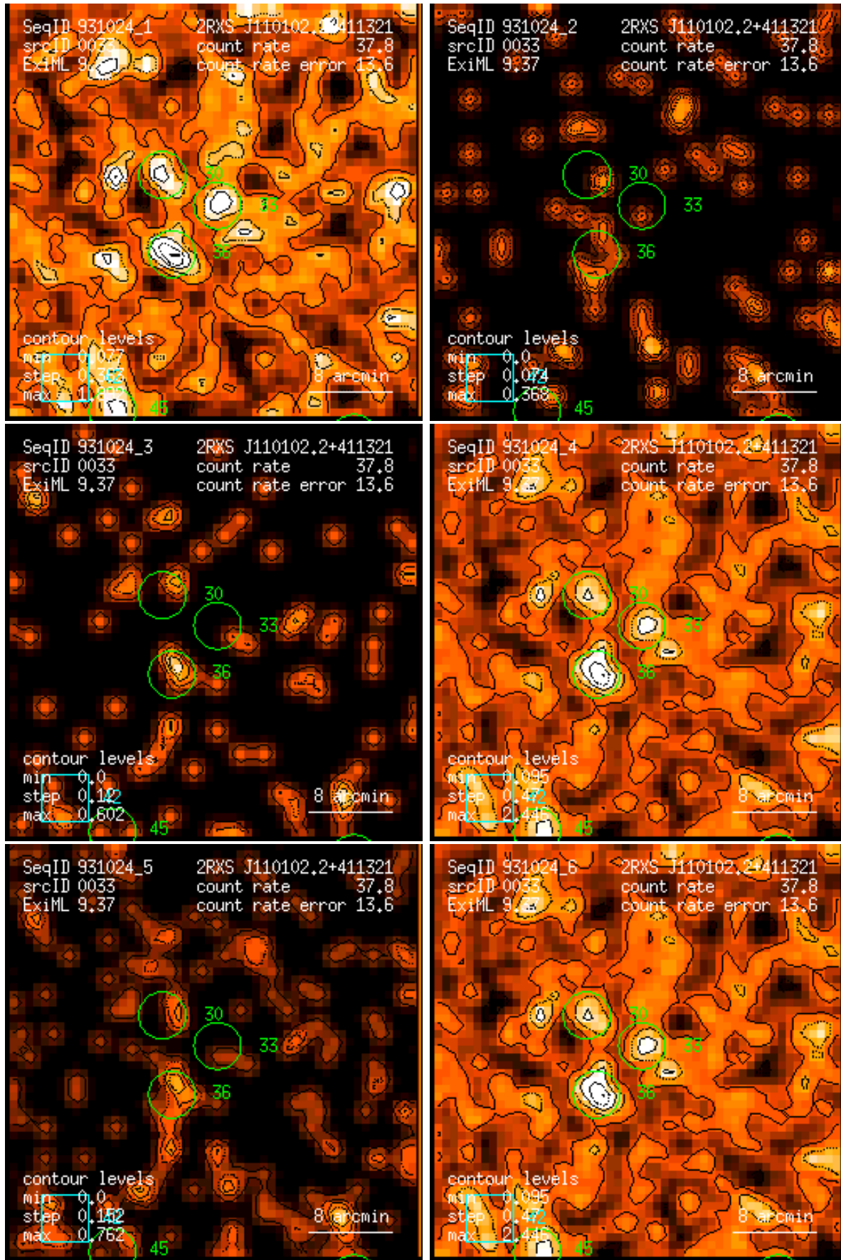
Figure 33: RASS 931024: detection 0033: band rate images, Gaussian filter: (1) PSPC channels 11 – 41, (2) 52 – 90, (3) 91 – 201, (4) 11 – 235, (5) 52 – 201, (6) 11 – 201. Broad band rates in counts/ks. Band rate contour levels in counts/ks/arcmin 2 .
