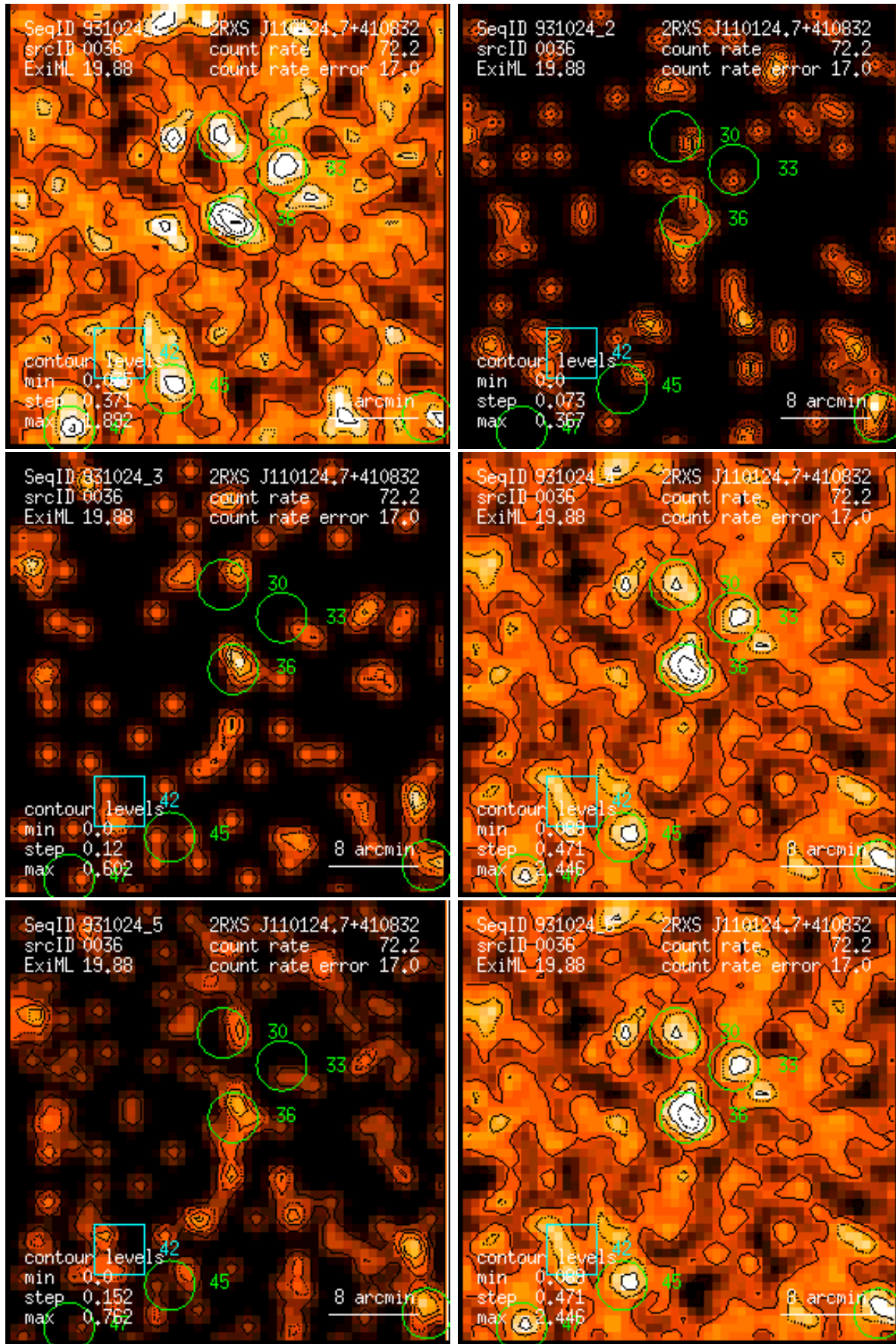
Figure 36: RASS 931024: detection 0036: band rate images, Gaussian filter: (1) PSPC channels 11 – 41, (2) 52 – 90, (3) 91 – 201, (4) 11 – 235, (5) 52 – 201, (6) 11 – 201. Broad band rates in counts/ks. Band rate contour levels in counts/ks/arcmin 2 .
