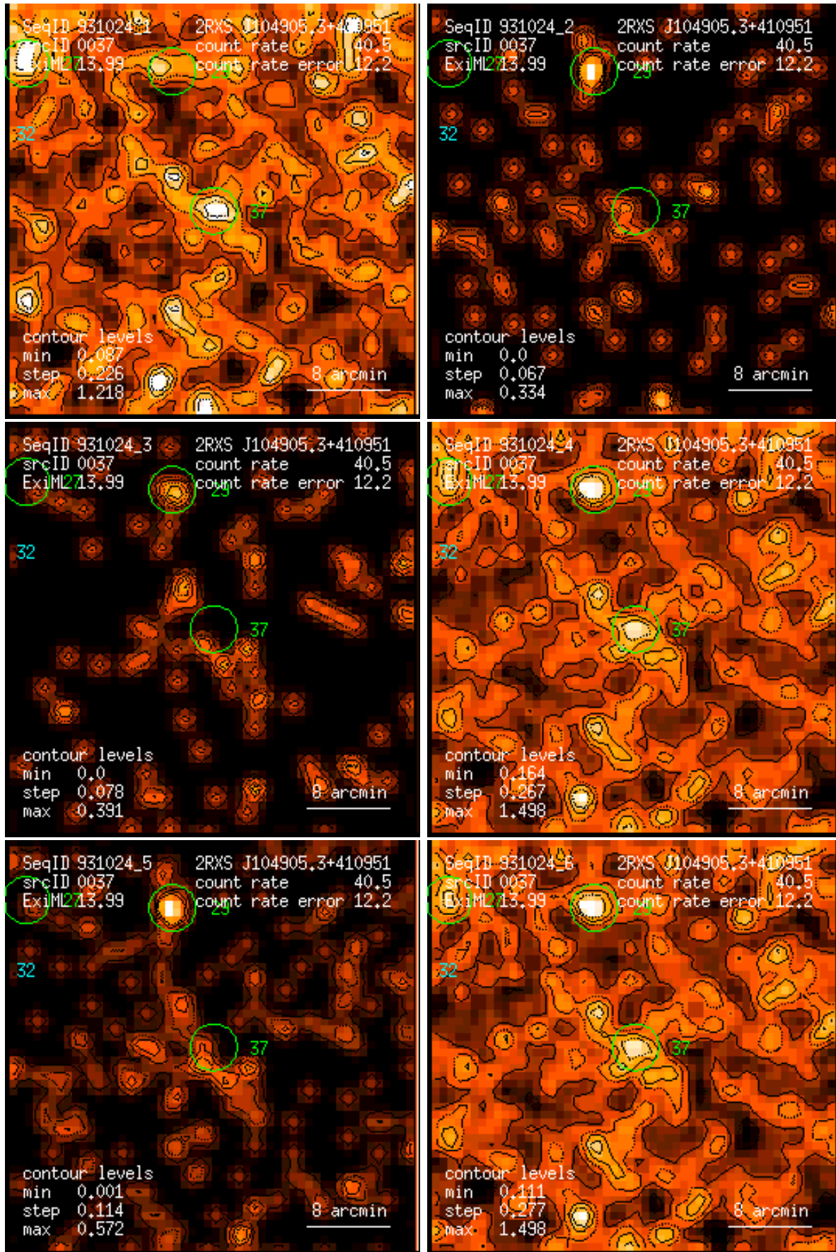
Figure 37: RASS 931024: detection 0037: band rate images, Gaussian filter: (1) PSPC channels 11 – 41, (2) 52 – 90, (3) 91 – 201, (4) 11 – 235, (5) 52 – 201, (6) 11 – 201. Broad band rates in counts/ks. Band rate contour levels in counts/ks/arcmin 2 .
