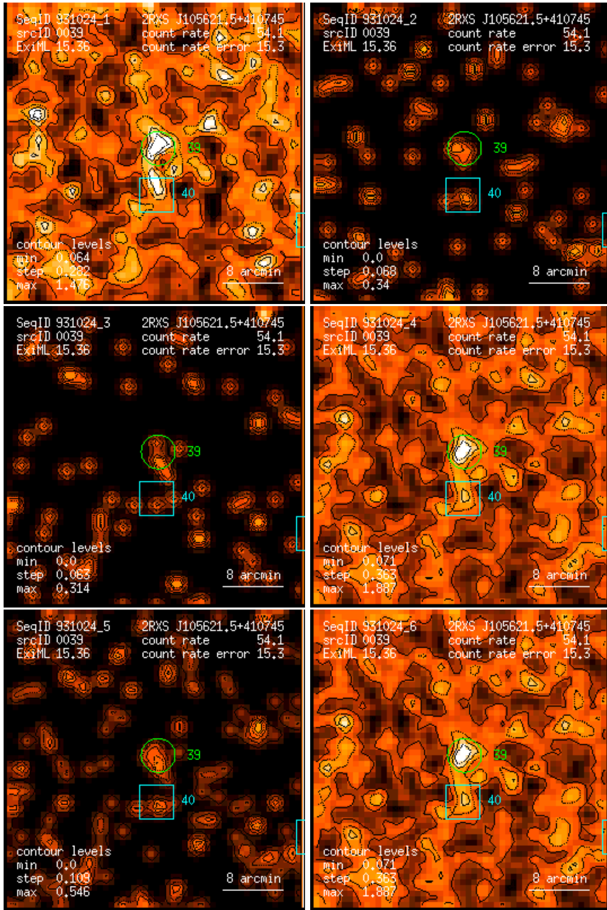
Figure 39: RASS 931024: detection 0039: band rate images, Gaussian filter: (1) PSPC channels 11 – 41, (2) 52 – 90, (3) 91 – 201, (4) 11 – 235, (5) 52 – 201, (6) 11 – 201. Broad band rates in counts/ks. Band rate contour levels in counts/ks/arcmin 2 .
