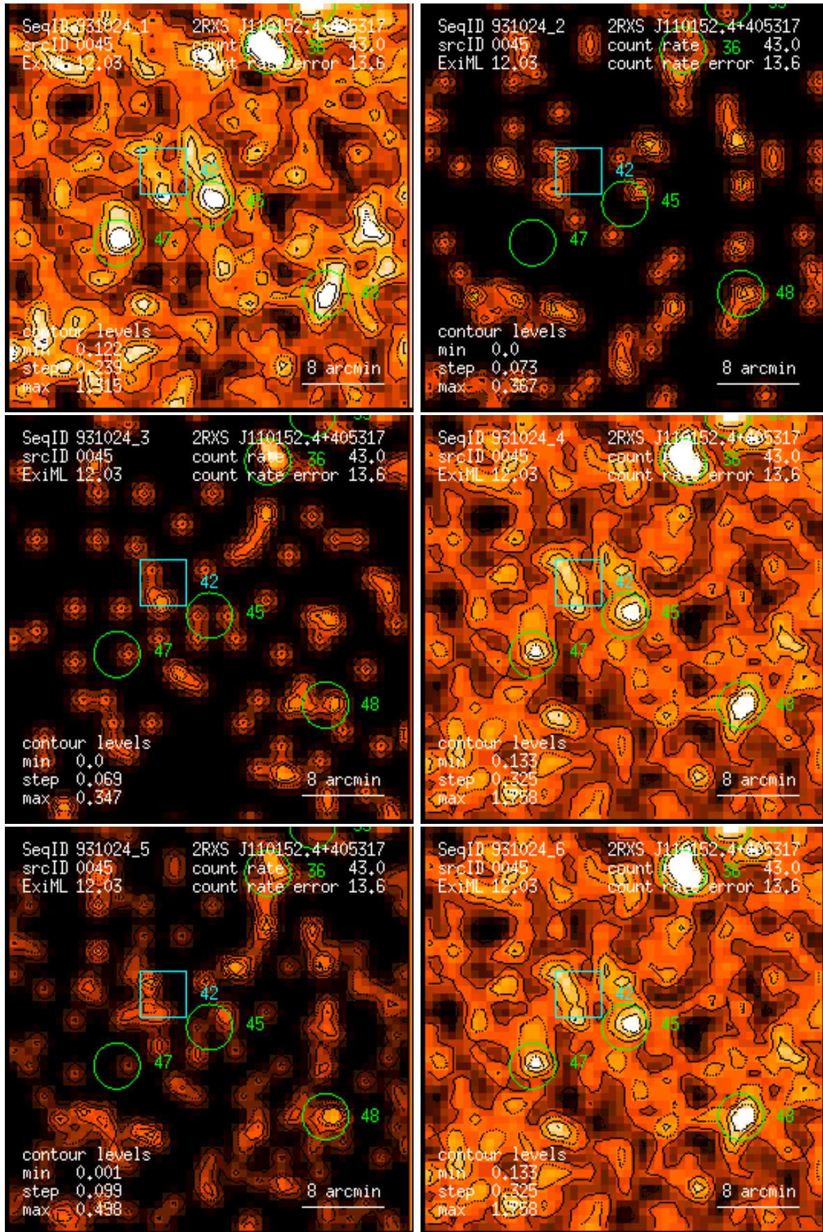
Figure 45: RASS 931024: detection 0045: band rate images, Gaussian filter: (1) PSPC channels 11 – 41, (2) 52 – 90, (3) 91 – 201, (4) 11 – 235, (5) 52 – 201, (6) 11 – 201. Broad band rates in counts/ks. Band rate contour levels in counts/ks/arcmin 2 .
