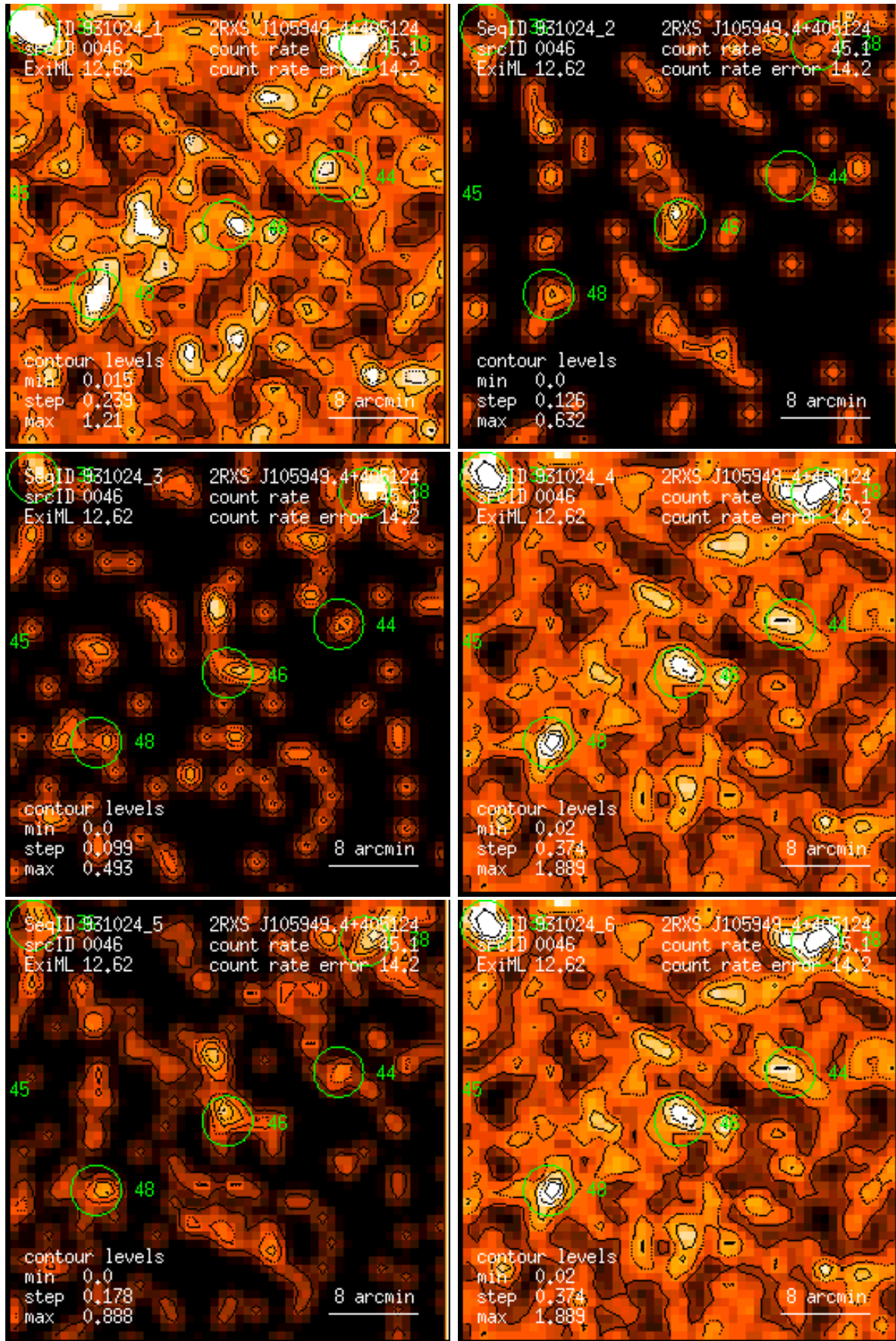
Figure 46: RASS 931024: detection 0046: band rate images, Gaussian filter: (1) PSPC channels 11 – 41, (2) 52 – 90, (3) 91 – 201, (4) 11 – 235, (5) 52 – 201, (6) 11 – 201. Broad band rates in counts/ks. Band rate contour levels in counts/ks/arcmin 2 .
