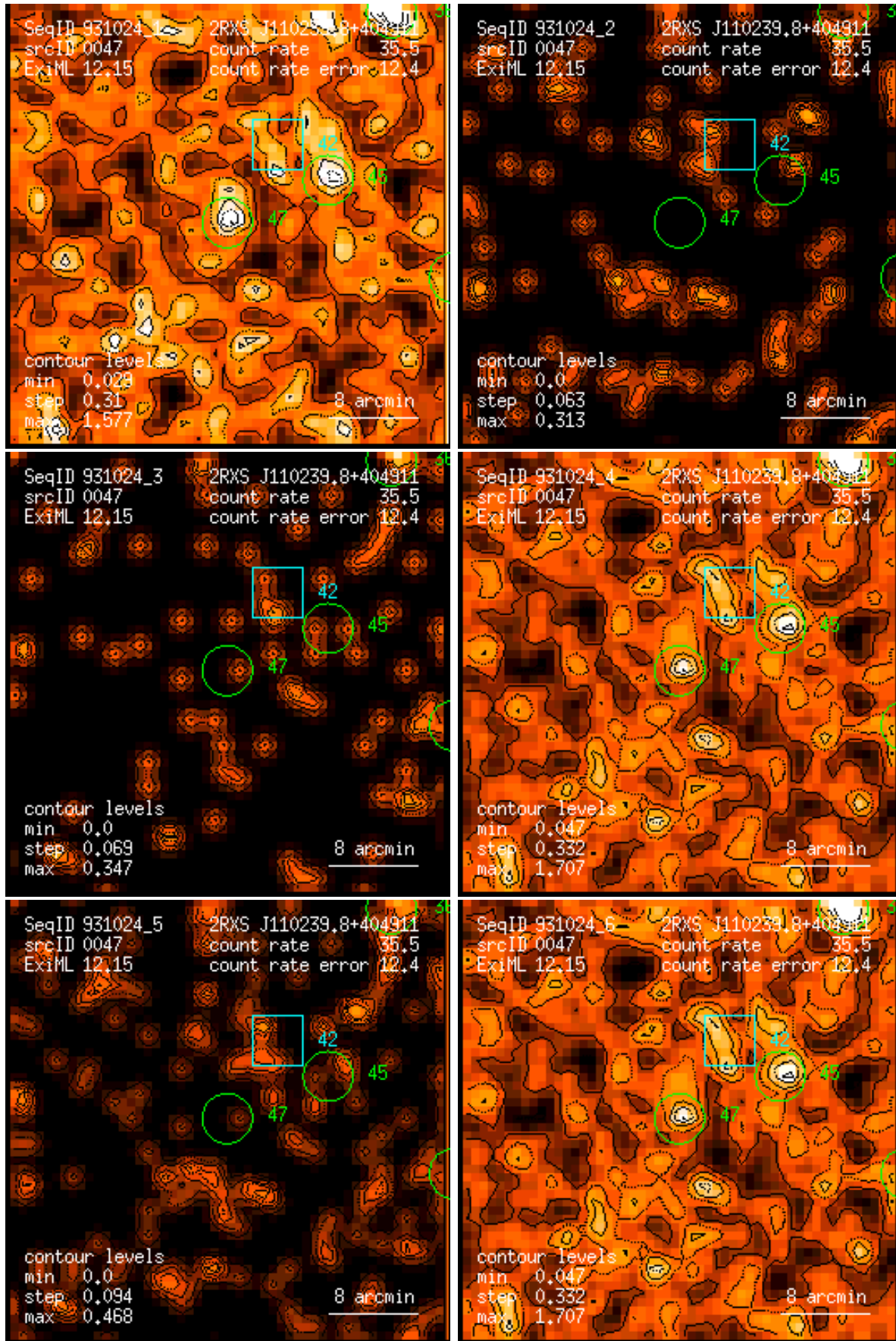
Figure 47: RASS 931024: detection 0047: band rate images, Gaussian filter: (1) PSPC channels 11 – 41, (2) 52 – 90, (3) 91 – 201, (4) 11 – 235, (5) 52 – 201, (6) 11 – 201. Broad band rates in counts/ks. Band rate contour levels in counts/ks/arcmin 2 .
