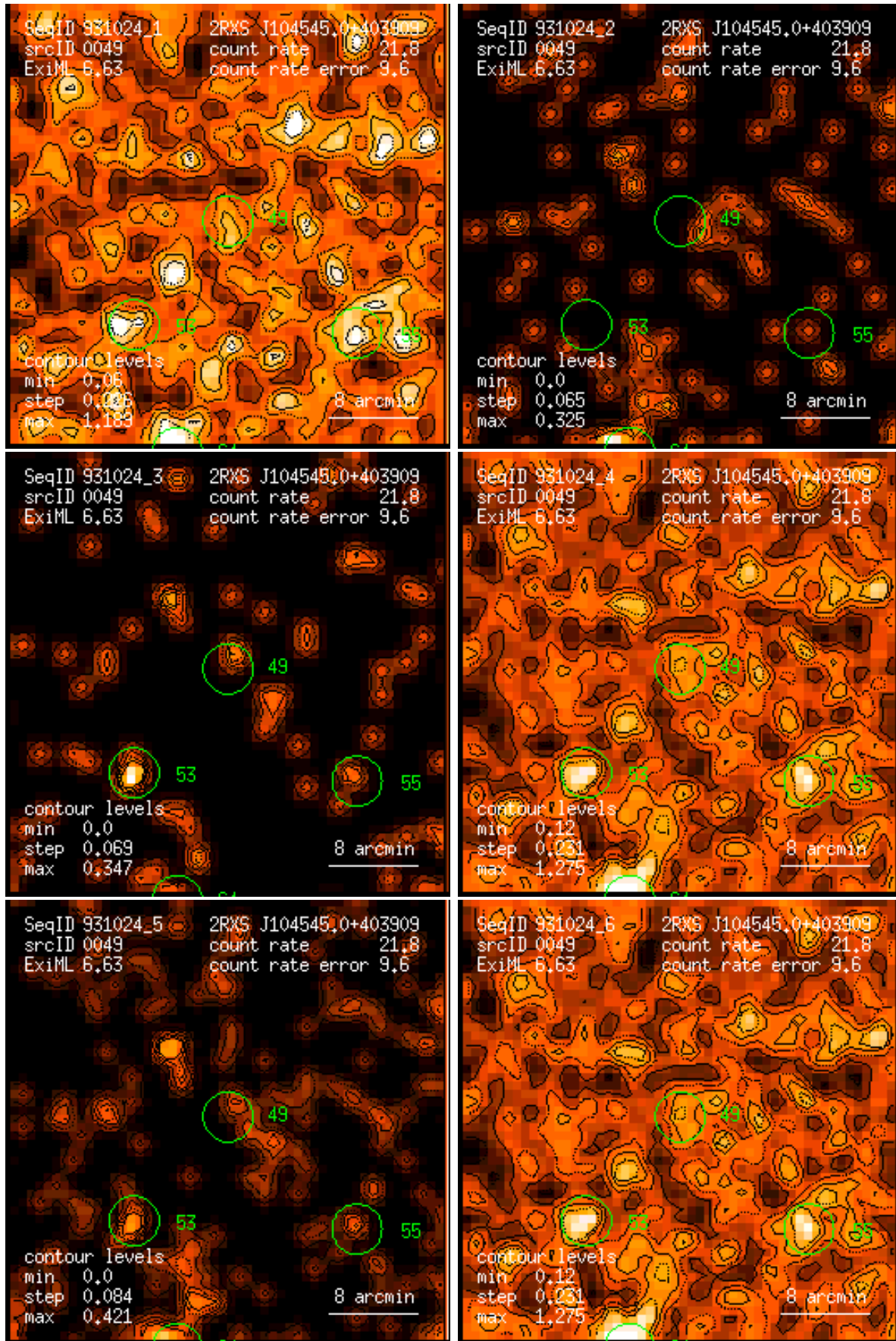
Figure 49: RASS 931024: detection 0049: band rate images, Gaussian filter: (1) PSPC channels 11 – 41, (2) 52 – 90, (3) 91 – 201, (4) 11 – 235, (5) 52 – 201, (6) 11 – 201. Broad band rates in counts/ks. Band rate contour levels in counts/ks/arcmin 2 .
