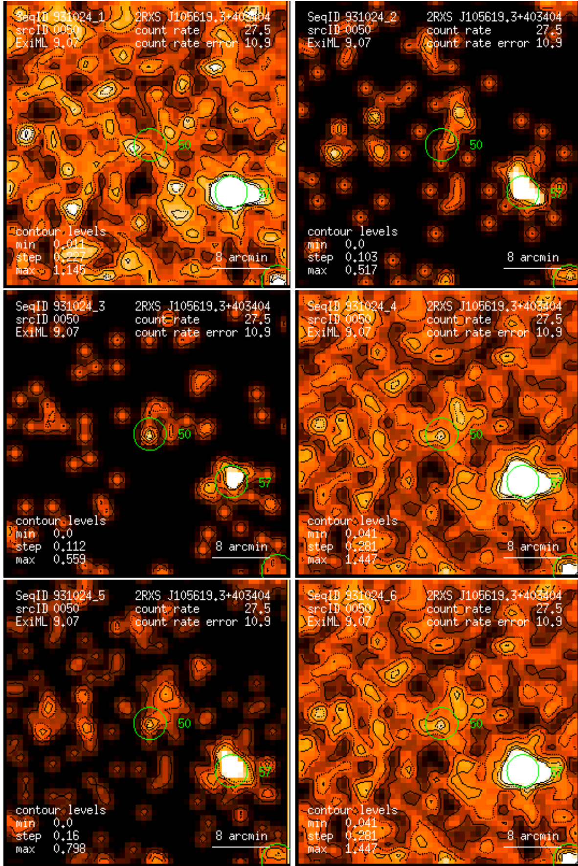
Figure 50: RASS 931024: detection 0050: band rate images, Gaussian filter: (1) PSPC channels 11 – 41, (2) 52 – 90, (3) 91 – 201, (4) 11 – 235, (5) 52 – 201, (6) 11 – 201. Broad band rates in counts/ks. Band rate contour levels in counts/ks/arcmin 2 .
