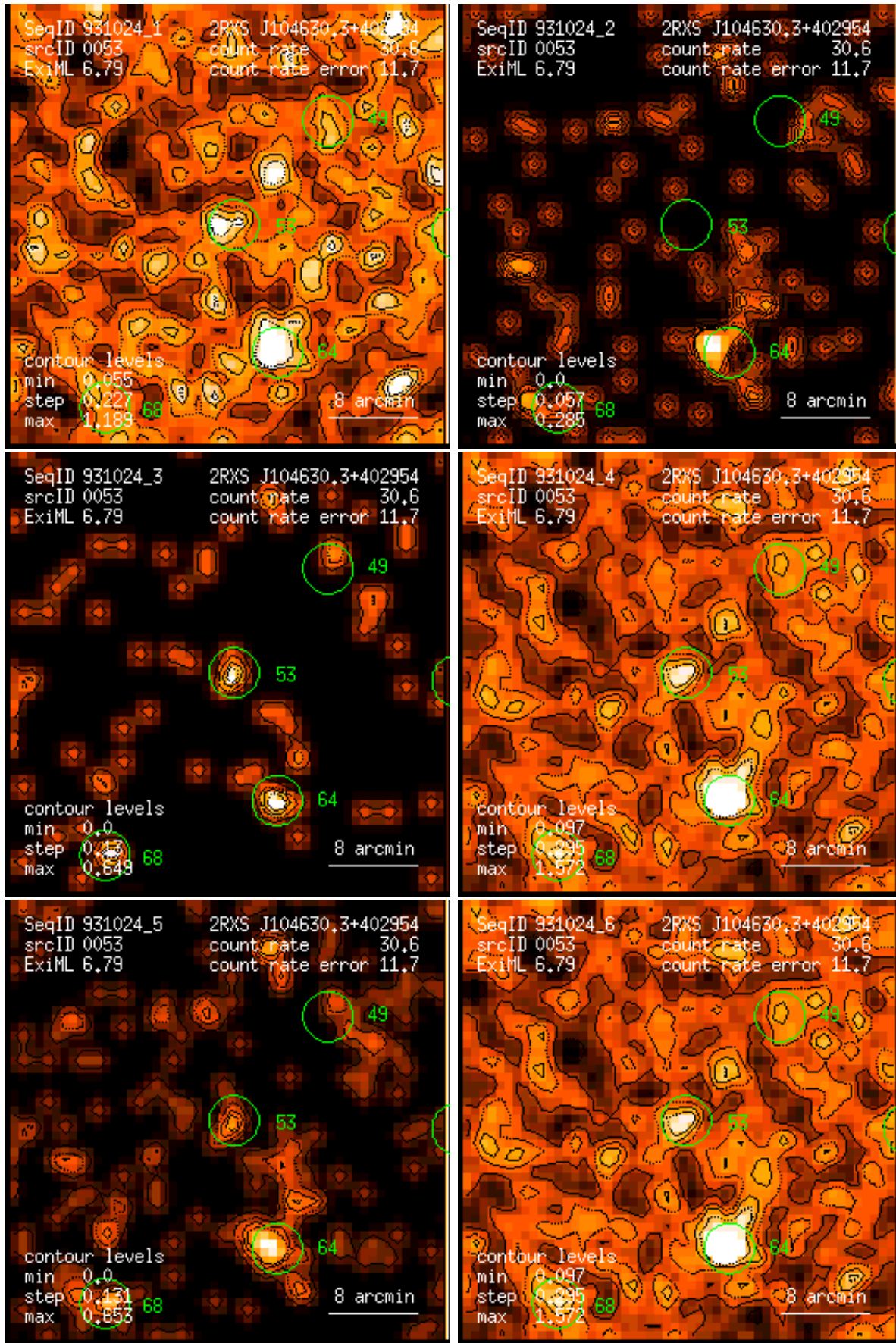
Figure 53: RASS 931024: detection 0053: band rate images, Gaussian filter: (1) PSPC channels 11 – 41, (2) 52 – 90, (3) 91 – 201, (4) 11 – 235, (5) 52 – 201, (6) 11 – 201. Broad band rates in counts/ks. Band rate contour levels in counts/ks/arcmin 2 .
