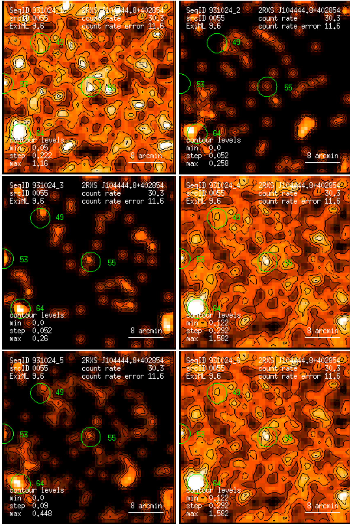
Figure 55: RASS 931024: detection 0055: band rate images, Gaussian filter: (1) PSPC channels 11 – 41, (2) 52 – 90, (3) 91 – 201, (4) 11 – 235, (5) 52 – 201, (6) 11 – 201. Broad band rates in counts/ks. Band rate contour levels in counts/ks/arcmin 2 .
