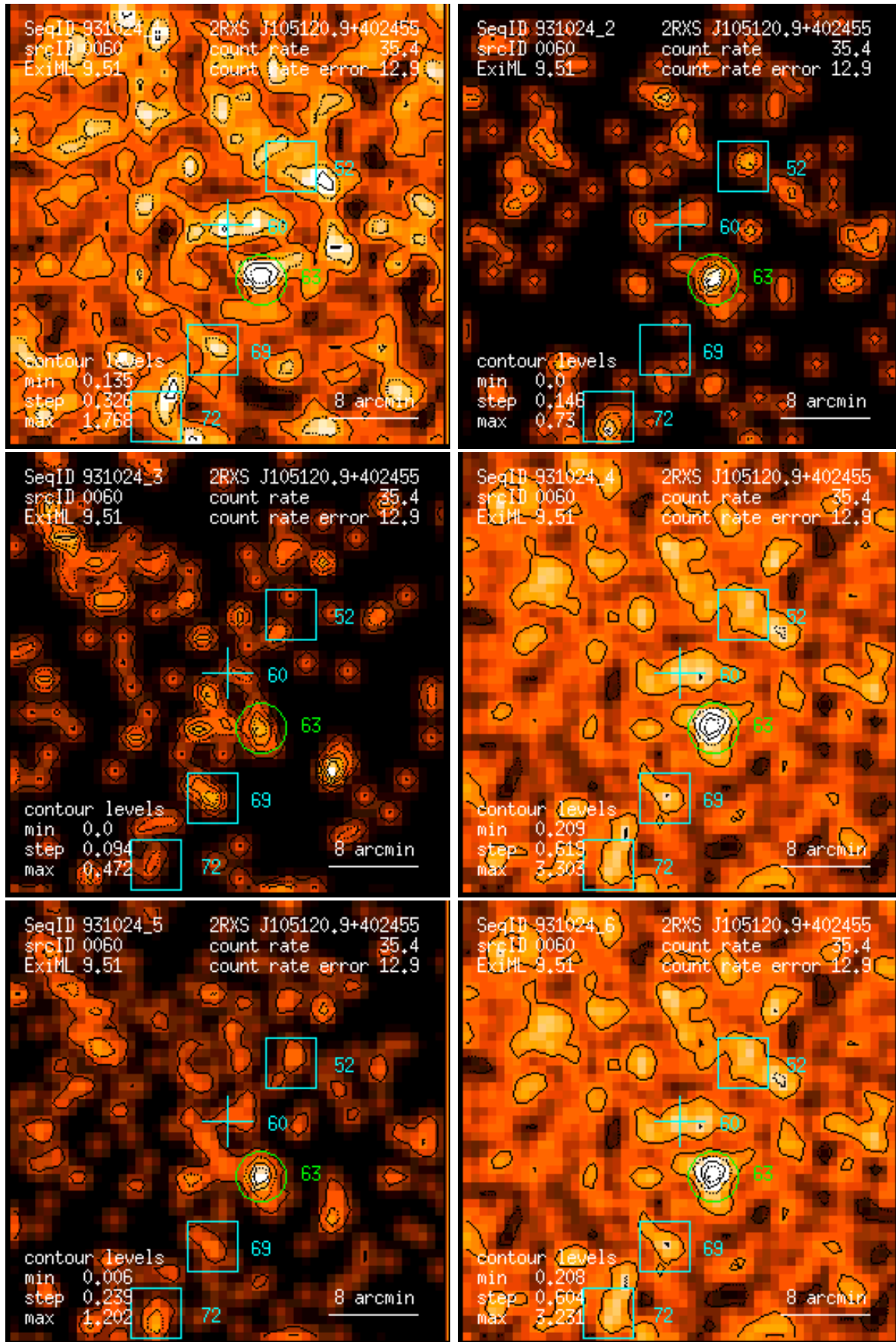
Figure 60: RASS 931024: detection 0060: band rate images, Gaussian filter: (1) PSPC channels 11 – 41, (2) 52 – 90, (3) 91 – 201, (4) 11 – 235, (5) 52 – 201, (6) 11 – 201. Broad band rates in counts/ks. Band rate contour levels in counts/ks/arcmin 2 .
