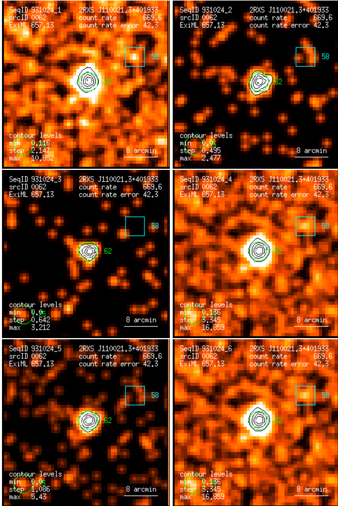
Figure 62: RASS 931024: detection 0062: band rate images, Gaussian filter: (1) PSPC channels 11 – 41, (2) 52 – 90, (3) 91 – 201, (4) 11 – 235, (5) 52 – 201, (6) 11 – 201. Broad band rates in counts/ks. Band rate contour levels in counts/ks/arcmin 2 .
