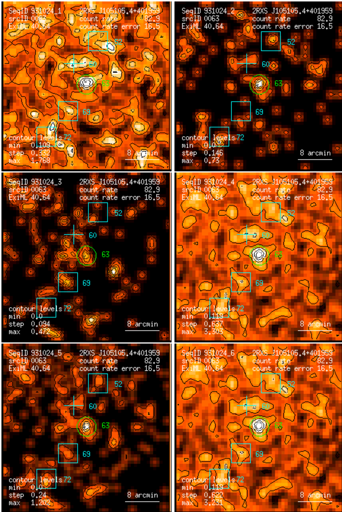
Figure 63: RASS 931024: detection 0063: band rate images, Gaussian filter: (1) PSPC channels 11 – 41, (2) 52 – 90, (3) 91 – 201, (4) 11 – 235, (5) 52 – 201, (6) 11 – 201. Broad band rates in counts/ks. Band rate contour levels in counts/ks/arcmin 2 .
