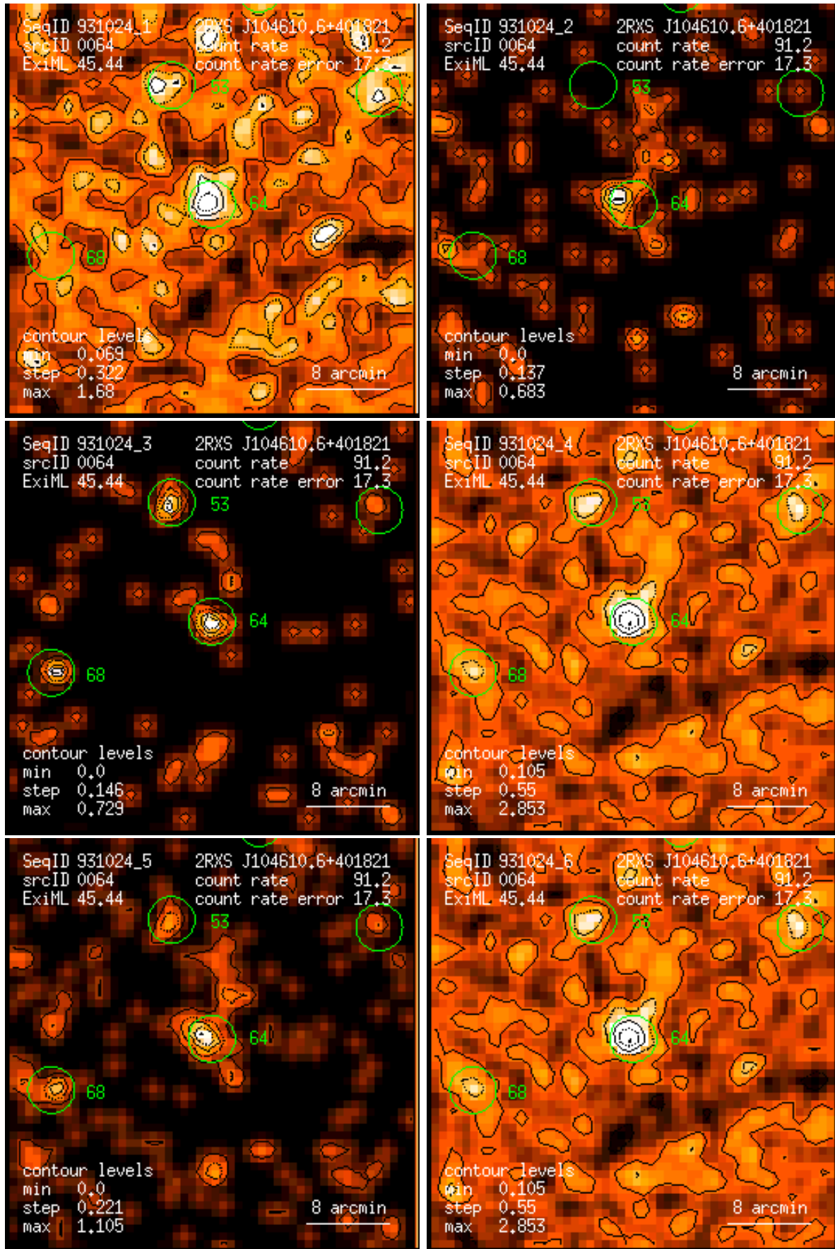
Figure 64: RASS 931024: detection 0064: band rate images, Gaussian filter: (1) PSPC channels 11 – 41, (2) 52 – 90, (3) 91 – 201, (4) 11 – 235, (5) 52 – 201, (6) 11 – 201. Broad band rates in counts/ks. Band rate contour levels in counts/ks/arcmin 2 .
