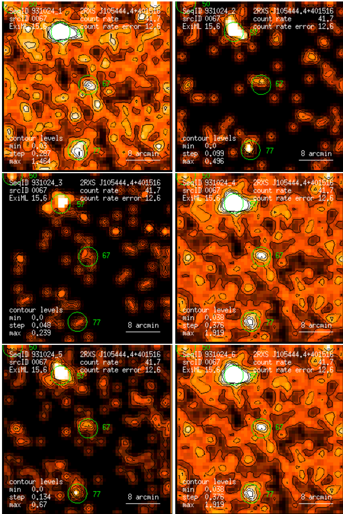
Figure 67: RASS 931024: detection 0067: band rate images, Gaussian filter: (1) PSPC channels 11 – 41, (2) 52 – 90, (3) 91 – 201, (4) 11 – 235, (5) 52 – 201, (6) 11 – 201. Broad band rates in counts/ks. Band rate contour levels in counts/ks/arcmin 2 .
