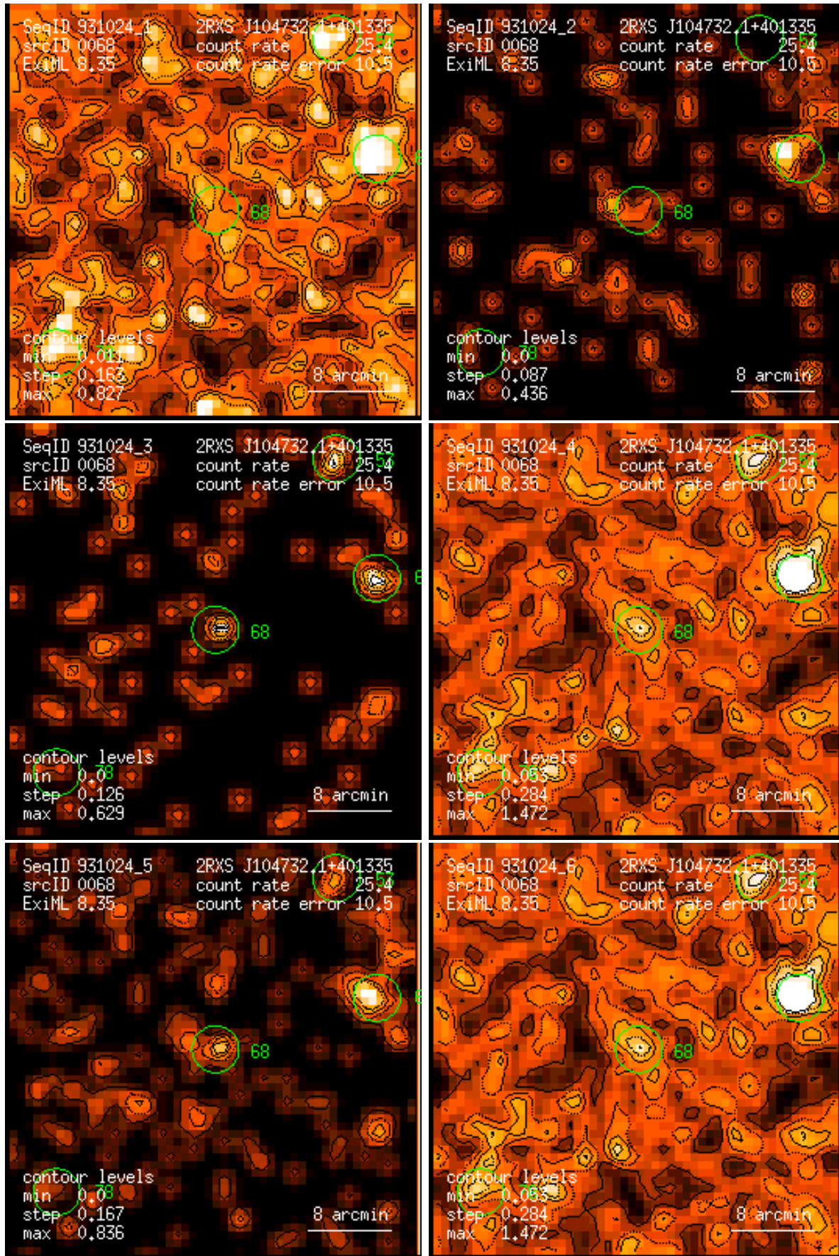
Figure 68: RASS 931024: detection 0068: band rate images, Gaussian filter: (1) PSPC channels 11 – 41, (2) 52 – 90, (3) 91 – 201, (4) 11 – 235, (5) 52 – 201, (6) 11 – 201. Broad band rates in counts/ks. Band rate contour levels in counts/ks/arcmin 2 .
