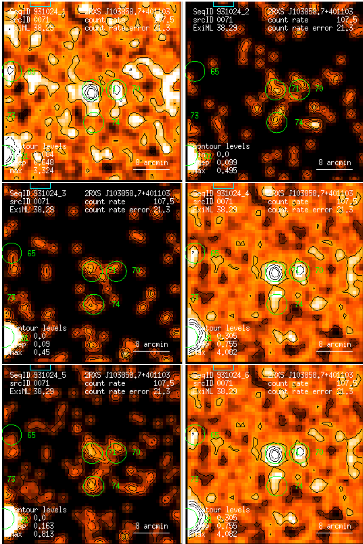
Figure 71: RASS 931024: detection 0071: band rate images, Gaussian filter: (1) PSPC channels 11 – 41, (2) 52 – 90, (3) 91 – 201, (4) 11 – 235, (5) 52 – 201, (6) 11 – 201. Broad band rates in counts/ks. Band rate contour levels in counts/ks/arcmin 2 .
