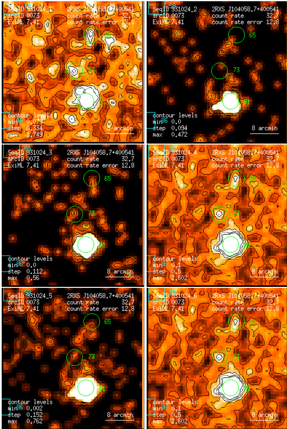
Figure 73: RASS 931024: detection 0073: band rate images, Gaussian filter: (1) PSPC channels 11 – 41, (2) 52 – 90, (3) 91 – 201, (4) 11 – 235, (5) 52 – 201, (6) 11 – 201. Broad band rates in counts/ks. Band rate contour levels in counts/ks/arcmin 2 .
