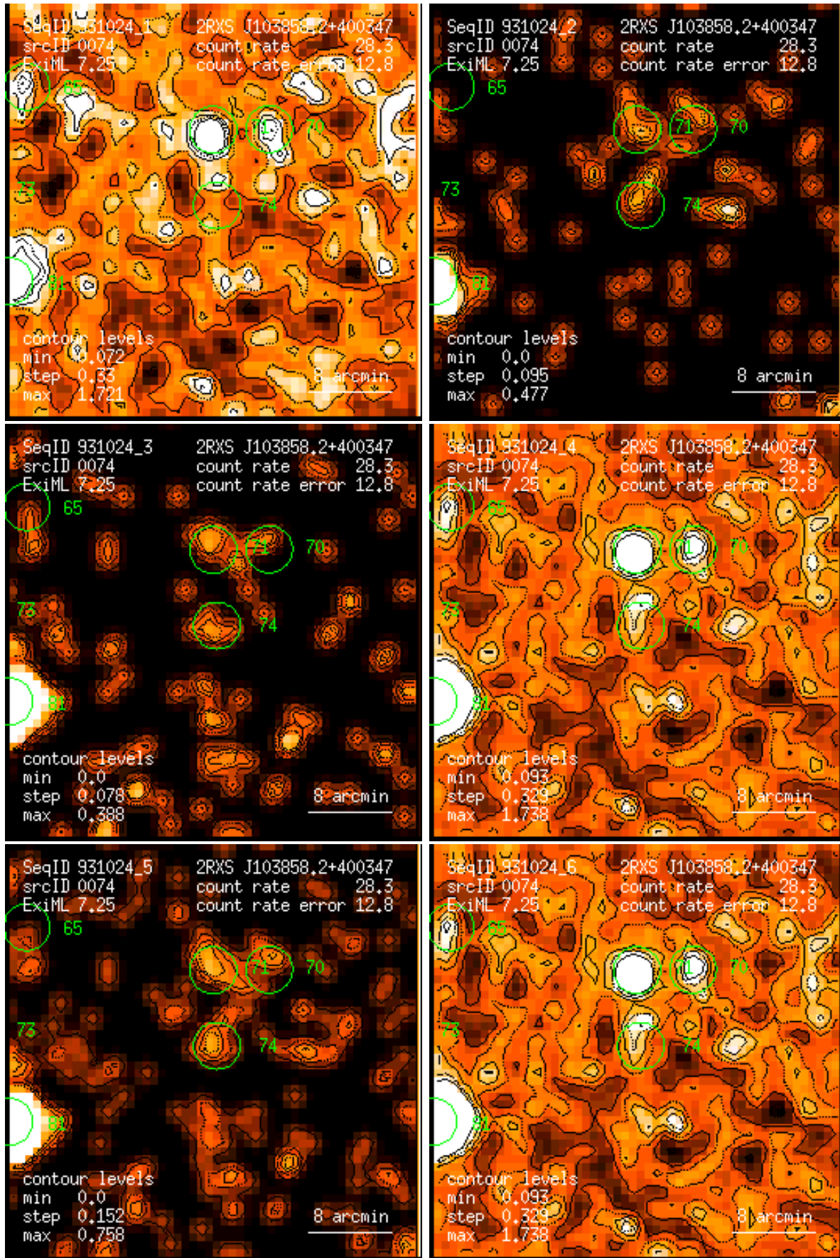
Figure 74: RASS 931024: detection 0074: band rate images, Gaussian filter: (1) PSPC channels 11 – 41, (2) 52 – 90, (3) 91 – 201, (4) 11 – 235, (5) 52 – 201, (6) 11 – 201. Broad band rates in counts/ks. Band rate contour levels in counts/ks/arcmin 2 .
