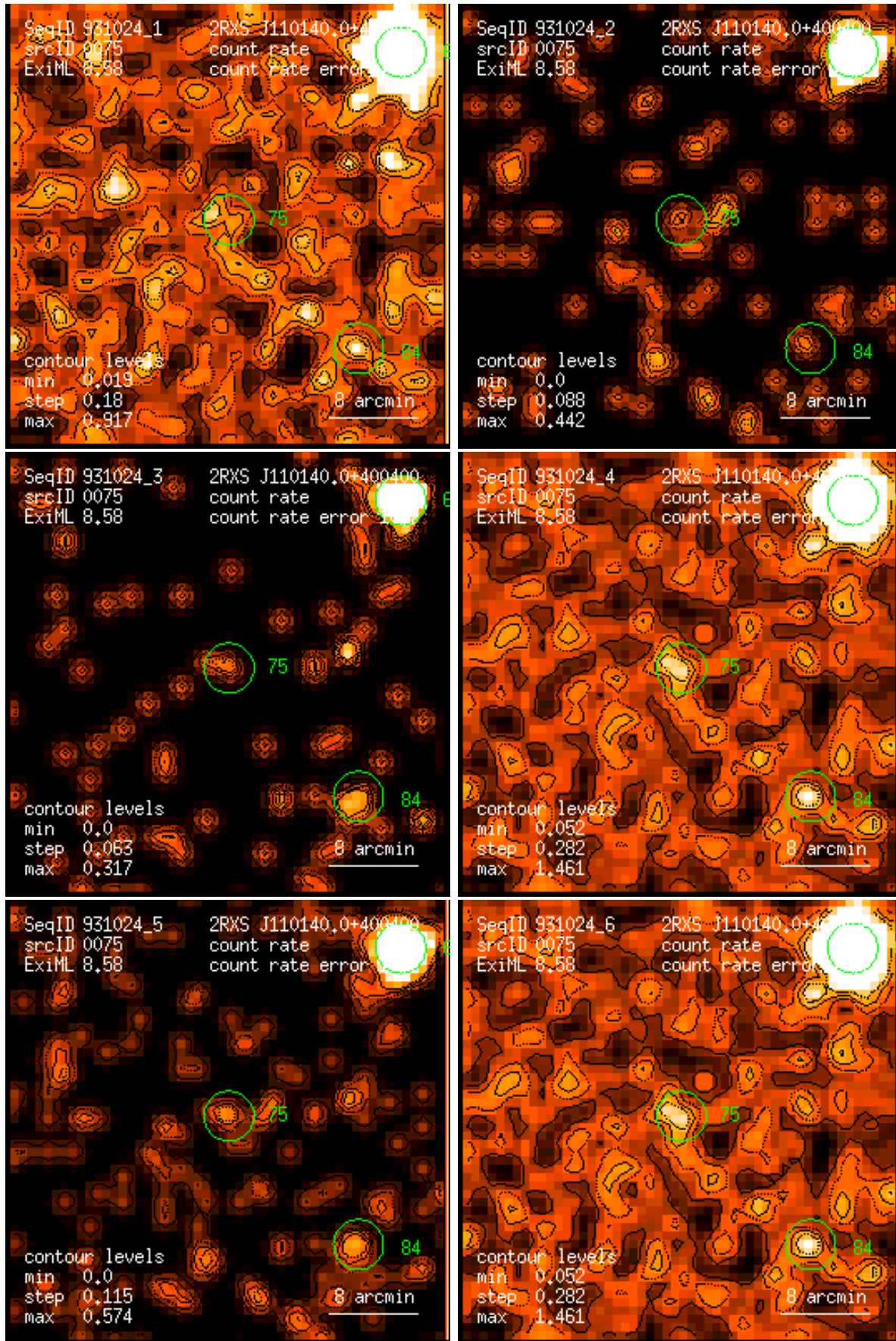
Figure 75: RASS 931024: detection 0075: band rate images, Gaussian filter: (1) PSPC channels 11 – 41, (2) 52 – 90, (3) 91 – 201, (4) 11 – 235, (5) 52 – 201, (6) 11 – 201. Broad band rates in counts/ks. Band rate contour levels in counts/ks/arcmin 2 .
