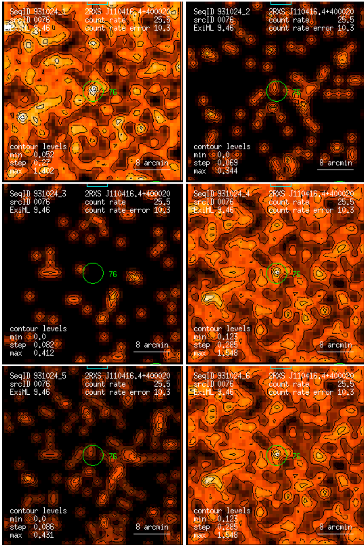
Figure 76: RASS 931024: detection 0076: band rate images, Gaussian filter: (1) PSPC channels 11 – 41, (2) 52 – 90, (3) 91 – 201, (4) 11 – 235, (5) 52 – 201, (6) 11 – 201. Broad band rates in counts/ks. Band rate contour levels in counts/ks/arcmin 2 .
