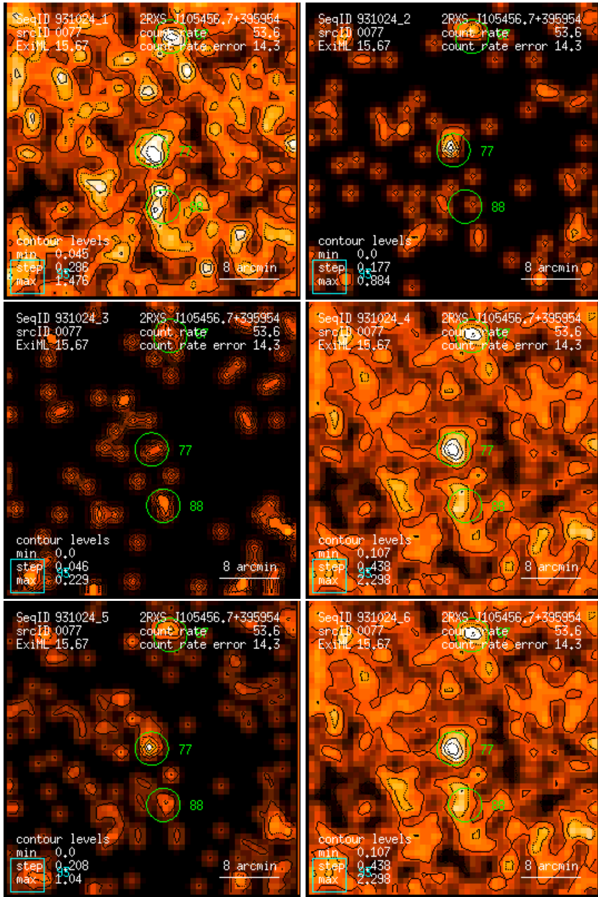
Figure 77: RASS 931024: detection 0077: band rate images, Gaussian filter: (1) PSPC channels 11 – 41, (2) 52 – 90, (3) 91 – 201, (4) 11 – 235, (5) 52 – 201, (6) 11 – 201. Broad band rates in counts/ks. Band rate contour levels in counts/ks/arcmin 2 .
