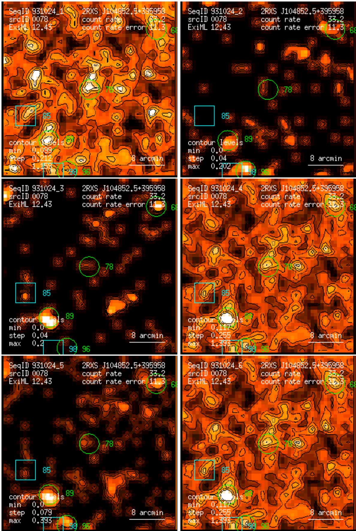
Figure 78: RASS 931024: detection 0078: band rate images, Gaussian filter: (1) PSPC channels 11 – 41, (2) 52 – 90, (3) 91 – 201, (4) 11 – 235, (5) 52 – 201, (6) 11 – 201. Broad band rates in counts/ks. Band rate contour levels in counts/ks/arcmin 2 .
