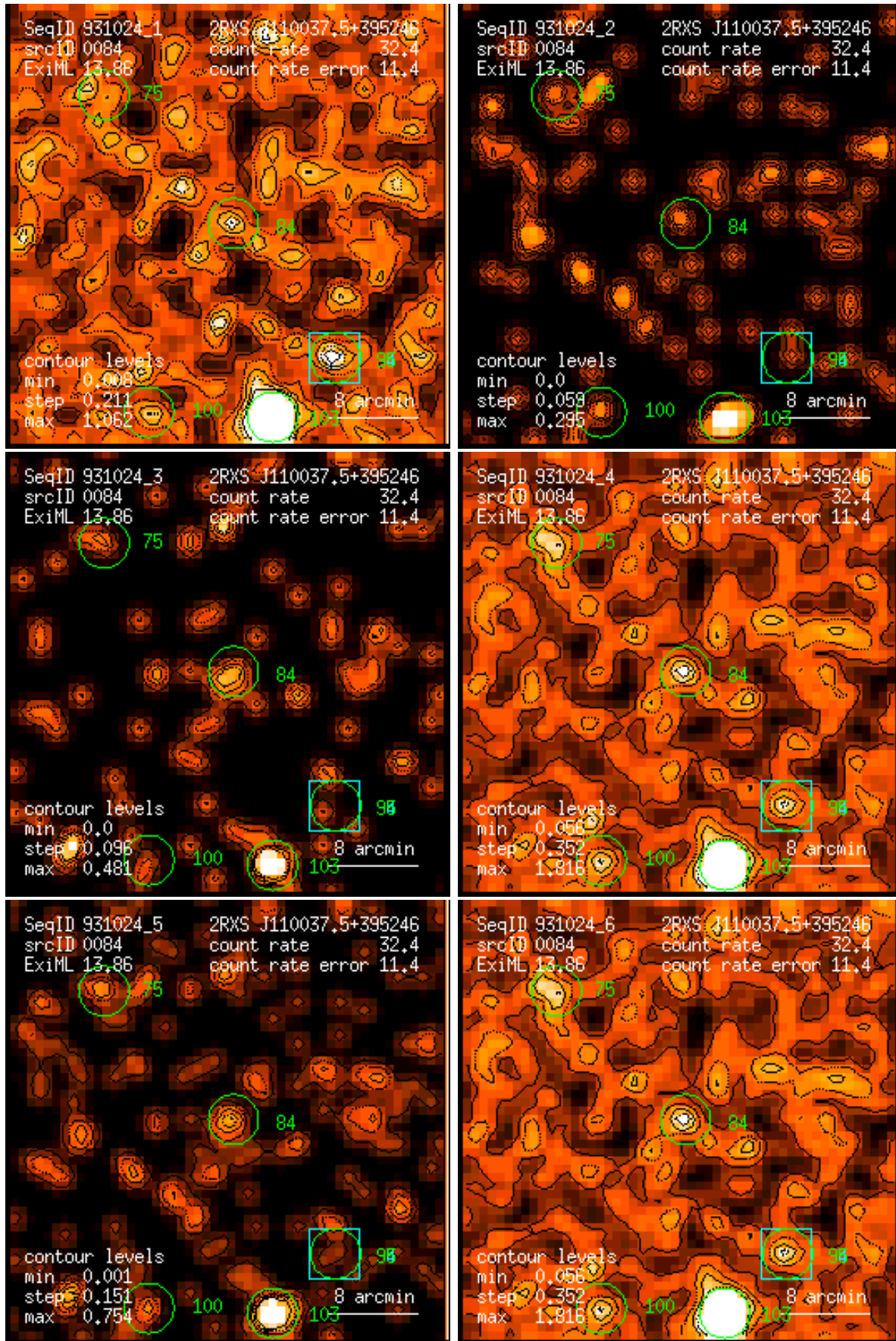
Figure 84: RASS 931024: detection 0084: band rate images, Gaussian filter: (1) PSPC channels 11 – 41, (2) 52 – 90, (3) 91 – 201, (4) 11 – 235, (5) 52 – 201, (6) 11 – 201. Broad band rates in counts/ks. Band rate contour levels in counts/ks/arcmin 2 .
