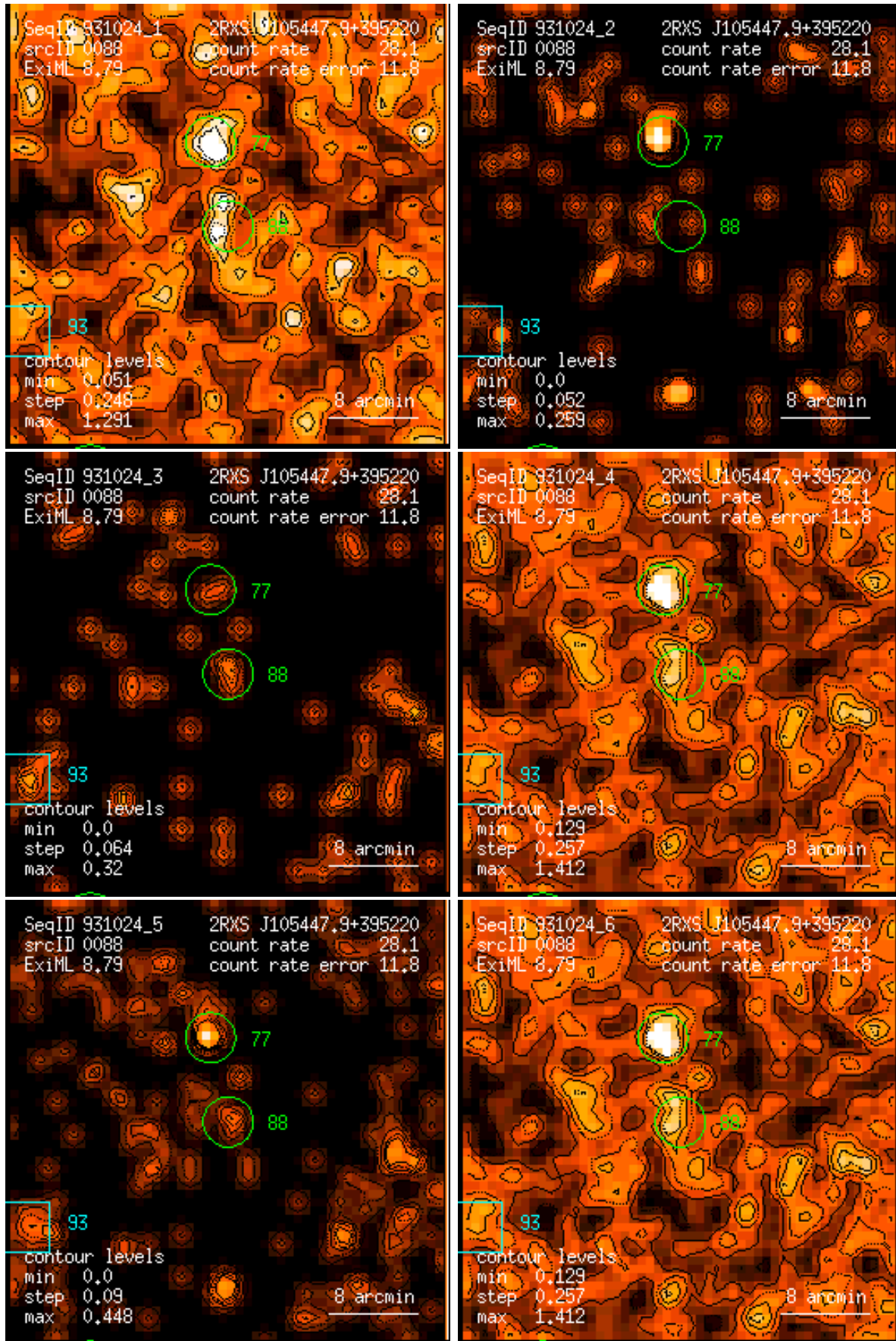
Figure 88: RASS 931024: detection 0088: band rate images, Gaussian filter: (1) PSPC channels 11 – 41, (2) 52 – 90, (3) 91 – 201, (4) 11 – 235, (5) 52 – 201, (6) 11 – 201. Broad band rates in counts/ks. Band rate contour levels in counts/ks/arcmin 2 .
