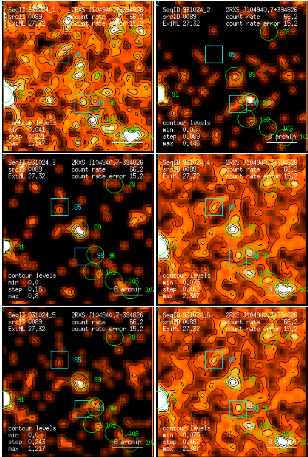
Figure 89: RASS 931024: detection 0089: band rate images, Gaussian filter: (1) PSPC channels 11 – 41, (2) 52 – 90, (3) 91 – 201, (4) 11 – 235, (5) 52 – 201, (6) 11 – 201. Broad band rates in counts/ks. Band rate contour levels in counts/ks/arcmin 2 .
