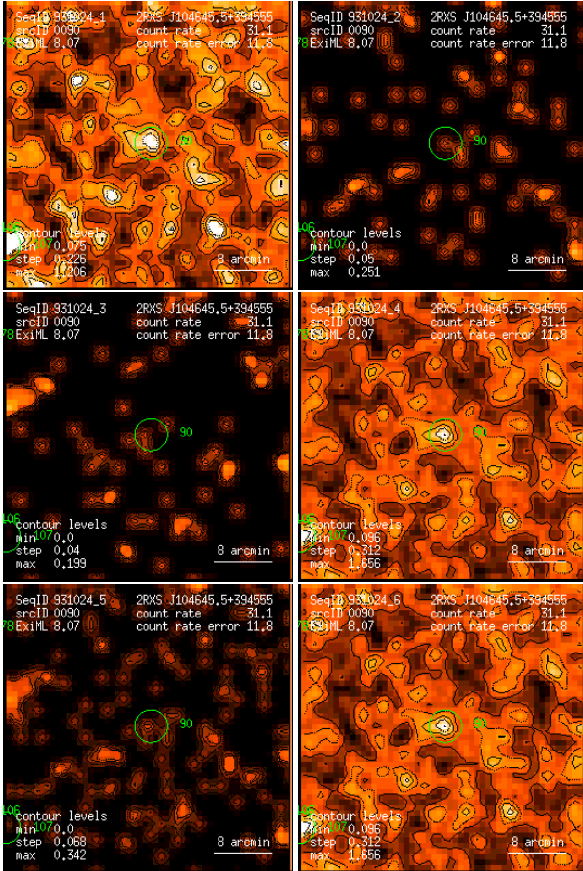
Figure 90: RASS 931024: detection 0090: band rate images, Gaussian filter: (1) PSPC channels 11 – 41, (2) 52 – 90, (3) 91 – 201, (4) 11 – 235, (5) 52 – 201, (6) 11 – 201. Broad band rates in counts/ks. Band rate contour levels in counts/ks/arcmin 2 .
