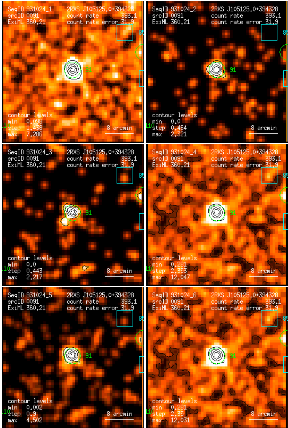
Figure 91: RASS 931024: detection 0091: band rate images, Gaussian filter: (1) PSPC channels 11 – 41, (2) 52 – 90, (3) 91 – 201, (4) 11 – 235, (5) 52 – 201, (6) 11 – 201. Broad band rates in counts/ks. Band rate contour levels in counts/ks/arcmin 2 .
