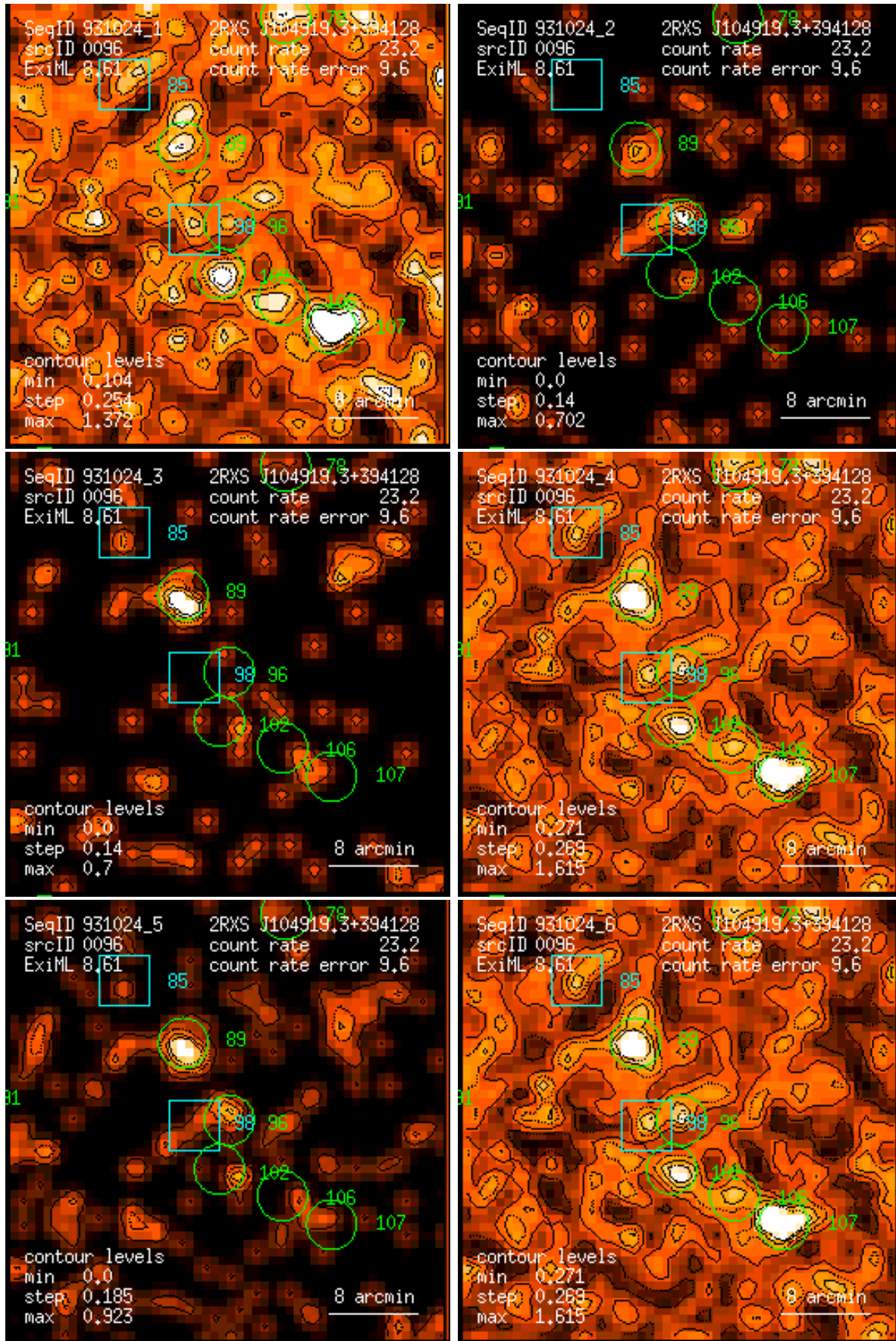
Figure 96: RASS 931024: detection 0096: band rate images, Gaussian filter: (1) PSPC channels 11 – 41, (2) 52 – 90, (3) 91 – 201, (4) 11 – 235, (5) 52 – 201, (6) 11 – 201. Broad band rates in counts/ks. Band rate contour levels in counts/ks/arcmin 2 .
