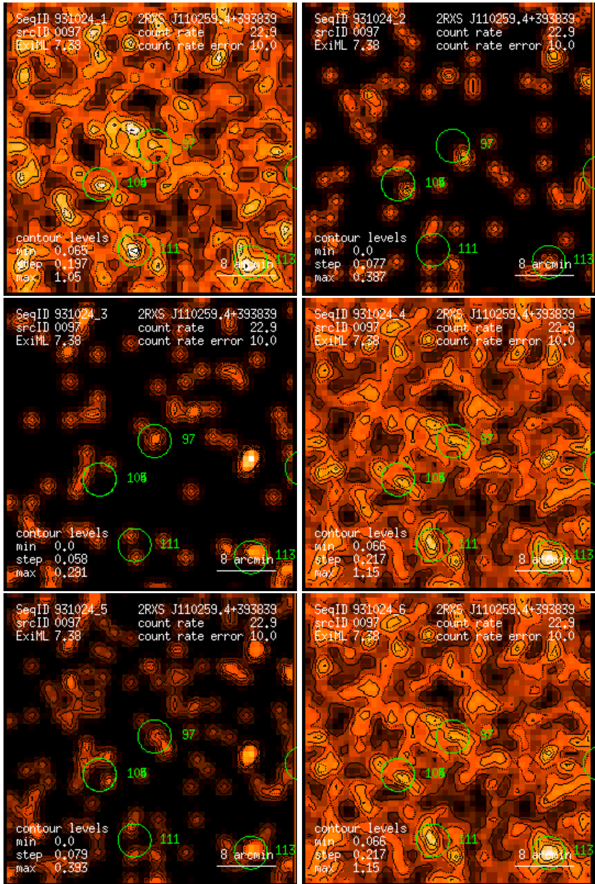
Figure 97: RASS 931024: detection 0097: band rate images, Gaussian filter: (1) PSPC channels 11 – 41, (2) 52 – 90, (3) 91 – 201, (4) 11 – 235, (5) 52 – 201, (6) 11 – 201. Broad band rates in counts/ks. Band rate contour levels in counts/ks/arcmin 2 .
