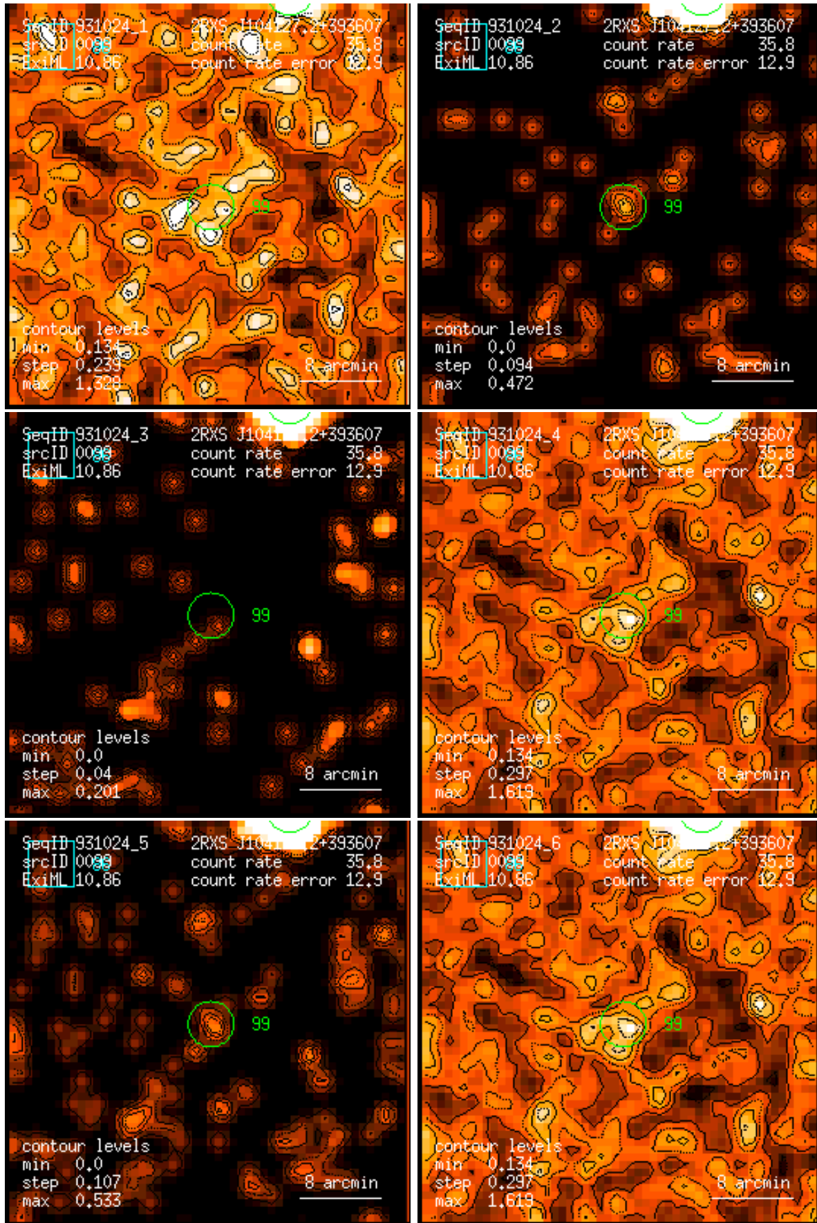
Figure 99: RASS 931024: detection 0099: band rate images, Gaussian filter: (1) PSPC channels 11 – 41, (2) 52 – 90, (3) 91 – 201, (4) 11 – 235, (5) 52 – 201, (6) 11 – 201. Broad band rates in counts/ks. Band rate contour levels in counts/ks/arcmin 2 .
