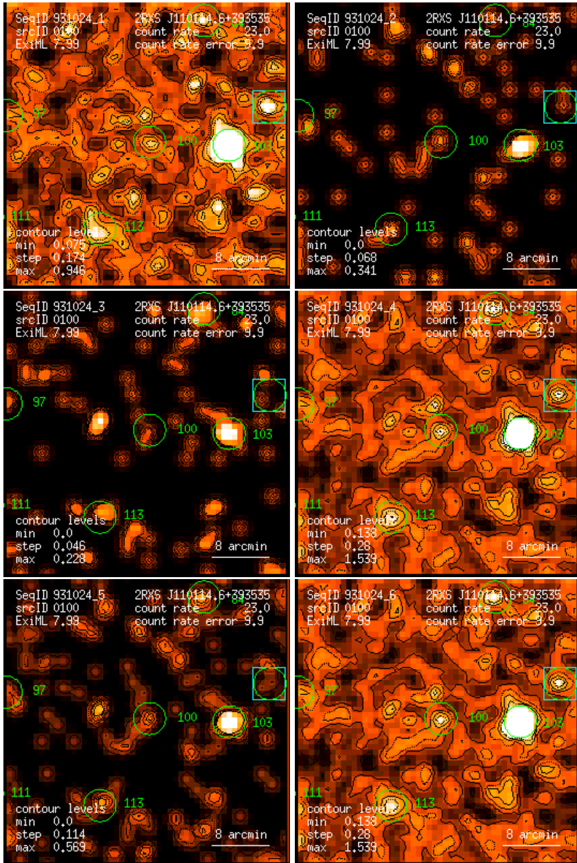
Figure 100: RASS 931024: detection 0100: band rate images, Gaussian filter: (1) PSPC channels 11 – 41, (2) 52 – 90, (3) 91 – 201, (4) 11 – 235, (5) 52 – 201, (6) 11 – 201. Broad band rates in counts/ks. Band rate contour levels in counts/ks/arcmin 2 .
