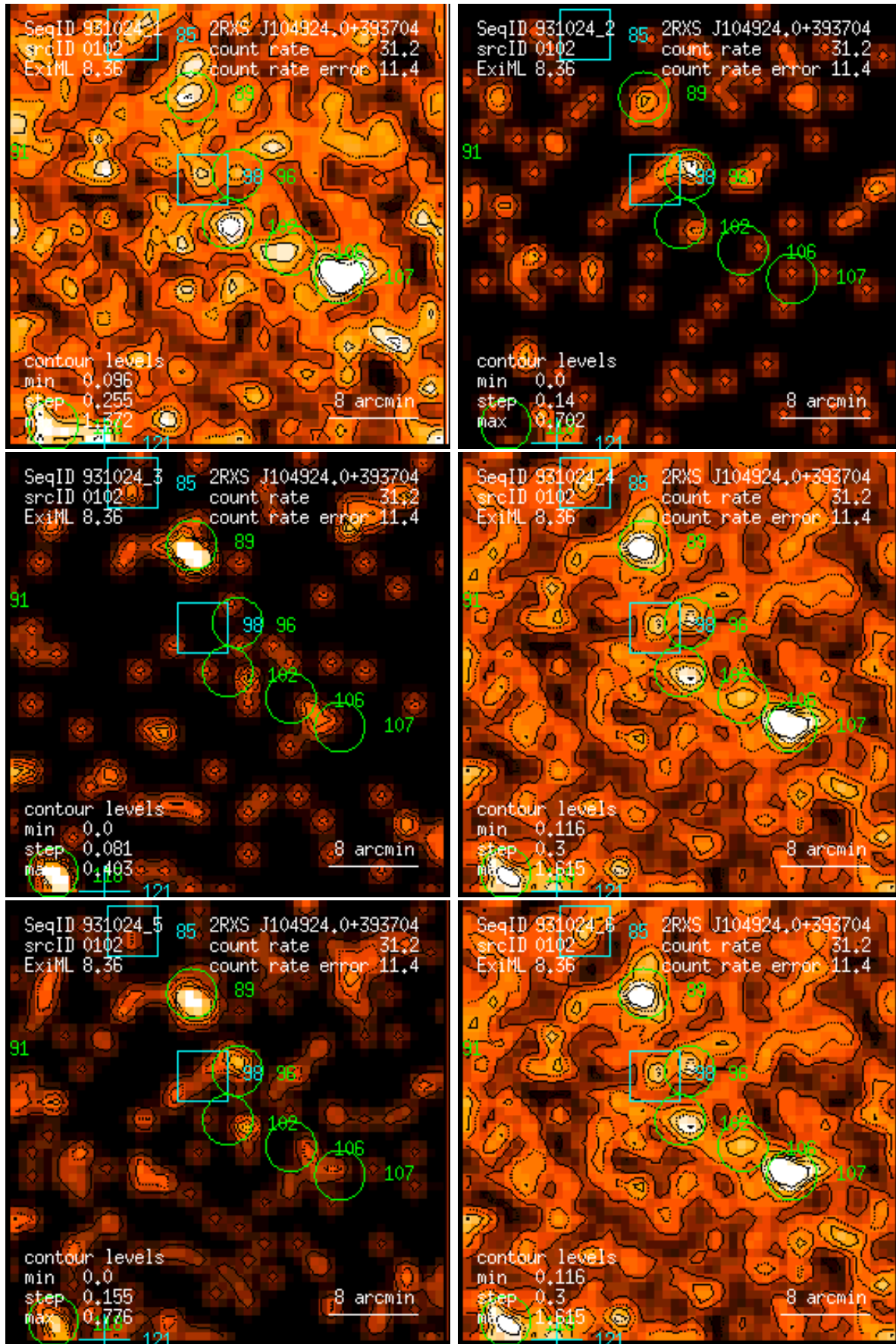
Figure 102: RASS 931024: detection 0102: band rate images, Gaussian filter: (1) PSPC channels 11 – 41, (2) 52 – 90, (3) 91 – 201, (4) 11 – 235, (5) 52 – 201, (6) 11 – 201. Broad band rates in counts/ks. Band rate contour levels in counts/ks/arcmin 2 .
